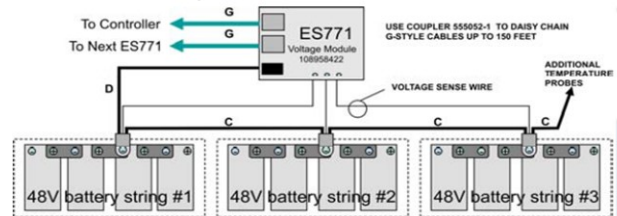
Battery Temperature and Voltage Measurement
