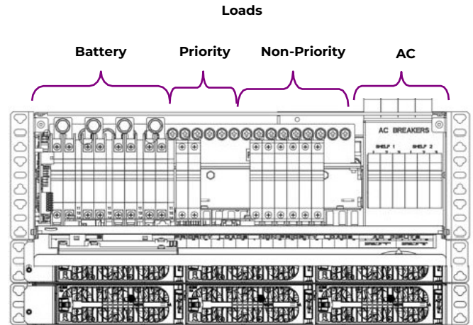
Two Shelf System
