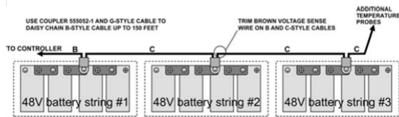
Battery Temperature Measurement
