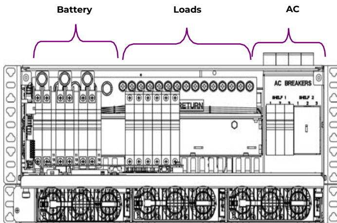
One Shelf System
