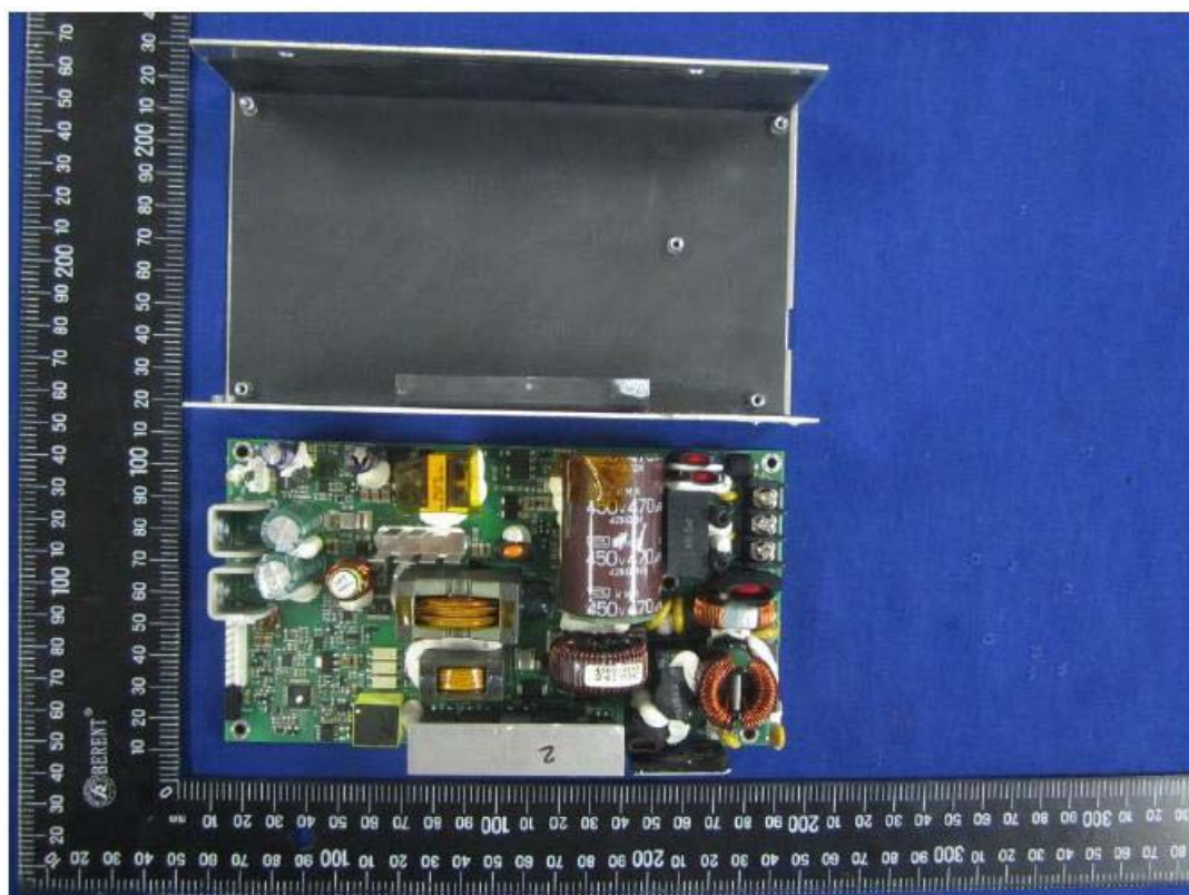
Picture 4 – Internal View
