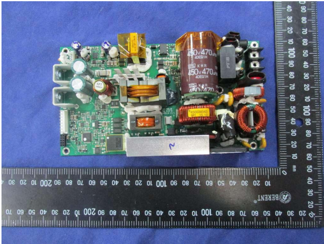
Picture 11 – Component side view of PCB
