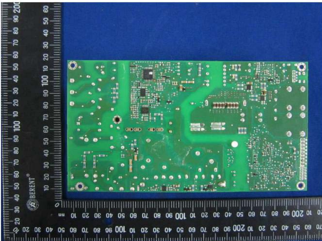
Picture 6 – Trace side view of PCB
