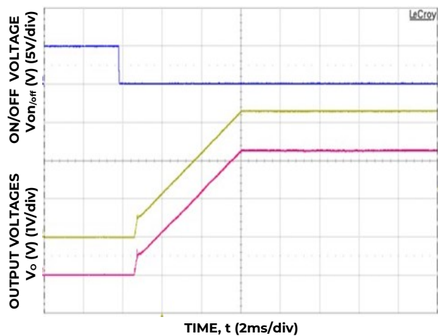
Figure 29. Typical Start-up Using On/Off Voltage ( V_{in} = 12\text{V} , I_o = I_{o1,max}, I_{o2,max} ).
