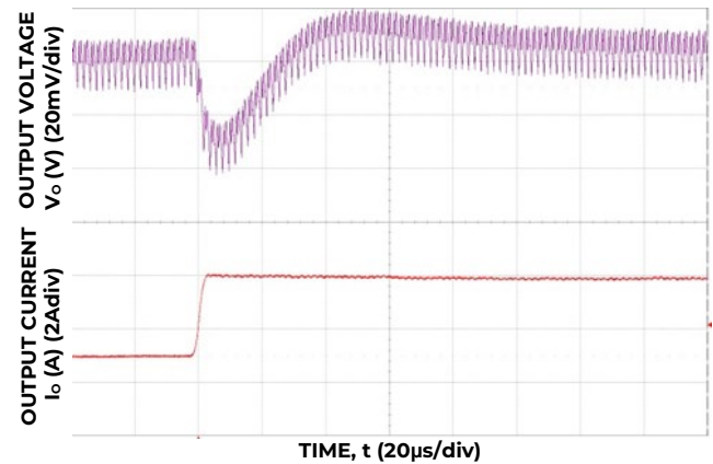
Figure 16. Transient Response to Dynamic Load Change on one output from 50% to 100% on at 12V in , C_{out} = 3 \times 47\mu F + 1 \times 330\mu F , C_{Tune} = 1800pF , R_{Tune} = 300\Omega
