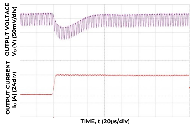
Figure 28. Transient Response to Dynamic Load Change on one output from 50% to 100% on at 12V in , C_{out} = 2 \times 47\mu\text{F} + 1 \times 330\mu\text{F} , C_{Tune} = 1200\text{pF} , R_{Tune} = 300\Omega
