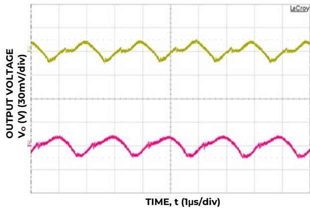
Figure 27. Typical output ripple and noise ( C_o = 2 \times 4.7\text{nF} + 2 \times 47\mu\text{F} ceramic, V_{in} = 12\text{V} , I_o = I_{o1,max}, I_{o2,max} ).
