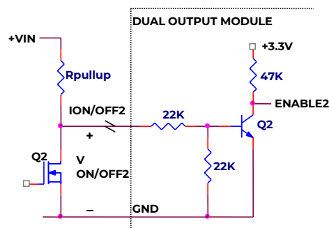
Figure 40. Circuit configuration for using negative On/Off logic.
