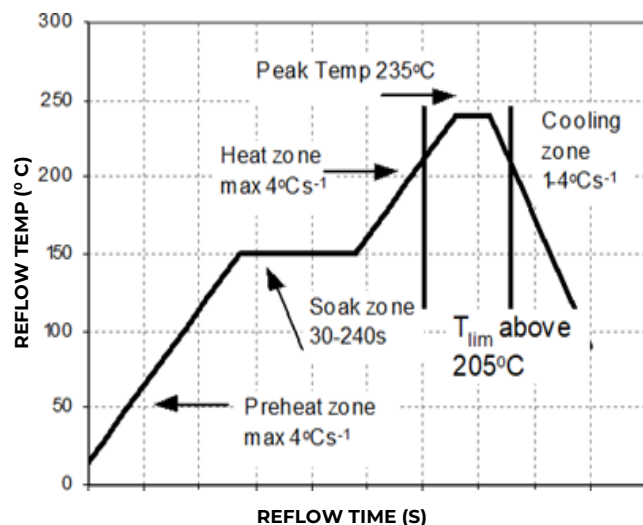
Figure 19. Recommended Reflow Profile for Sn/Pb solder.
