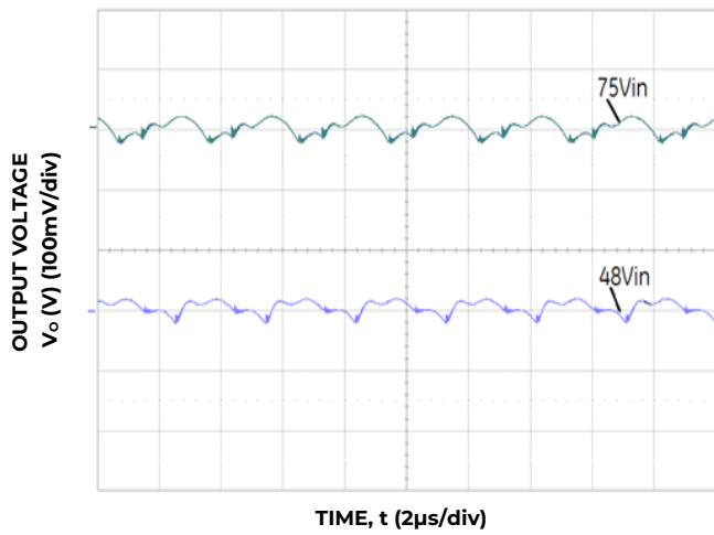
Figure 3. Typical output ripple and noise ( I_o = I_{o,max} ).
