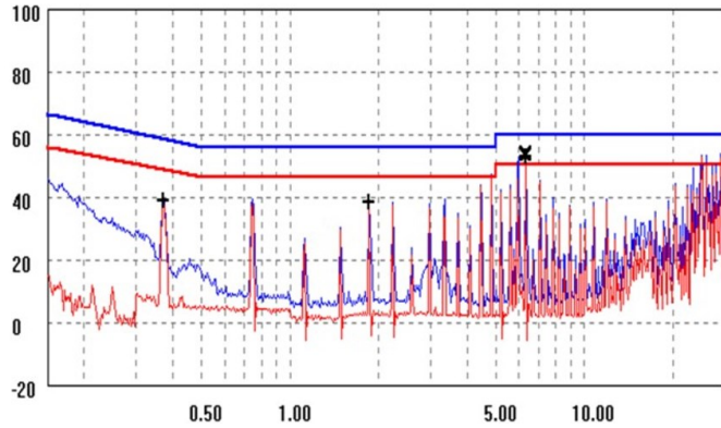
Figure 17. EMC signature using above filter
