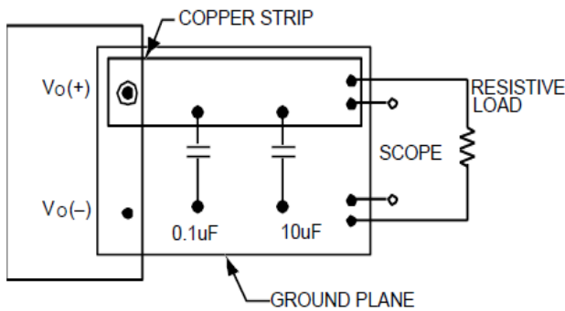
Figure 7. Input Reflected Ripple Current Test Setup.
