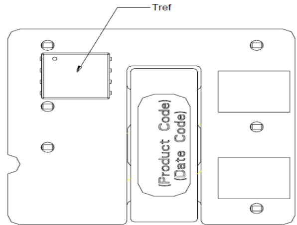
Figure 15. T_{ref} Temperature Measurement Location.
