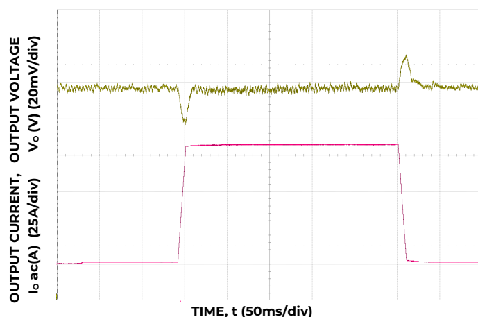
Figure 16. Trans. Resp. to 100A/μs Load Change from 25% to 75% at 12VIN, C_o=4 \times 0.047\mu\text{F} + 4 \times 0.1\mu\text{F} + 15 \times 22\mu\text{F} + 73 \times 47\mu\text{F} + 6 \times 470\mu\text{F} polymer
