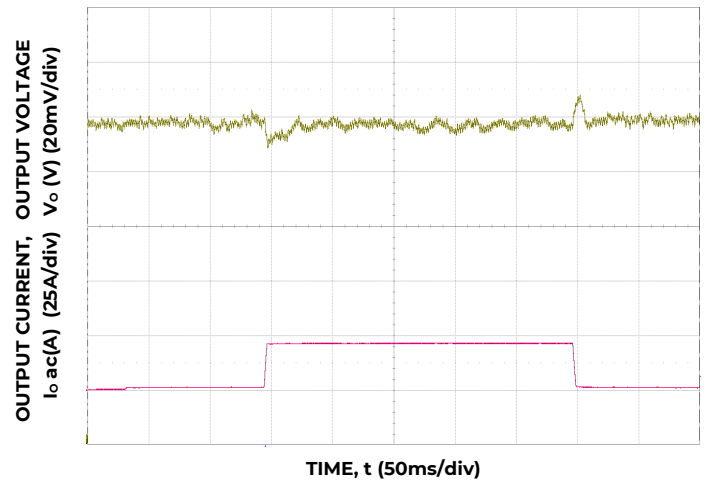
Figure 22. Trans. Resp. to 10A/μs Load Change from 25% to 75% at 12V IN , C_o = 4 \times 0.047\mu\text{F} + 4 \times 0.1\mu\text{F} + 15 \times 22\mu\text{F} + 73 \times 47\mu\text{F} + 6 \times 470\mu\text{F} polymer
