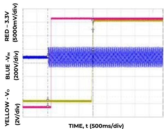
Figure 6. Typical Start-up ( V_{IN} = 150V_{ac} )
