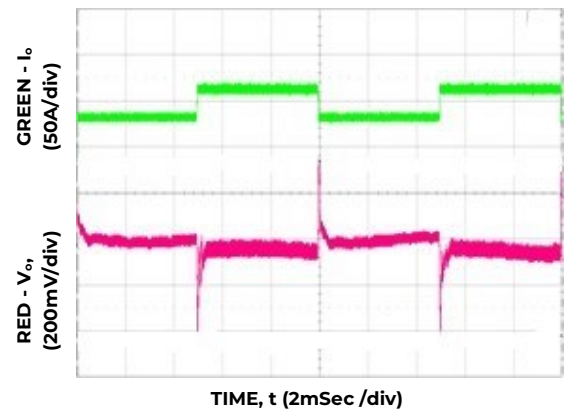
Figure 10. 50%-100%-50% Load Transient, Slew Rate = 1A/\mu S , V_{IN} = 230V_{ac} , V_o = 12V_{dc}
