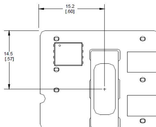
Figure 19. Pick and Place Location.
