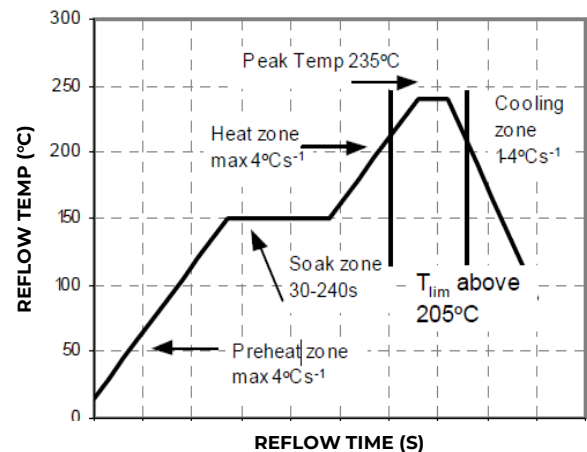
Figure 20. Recommended Reflow Profile for Sn/Pb solder.
