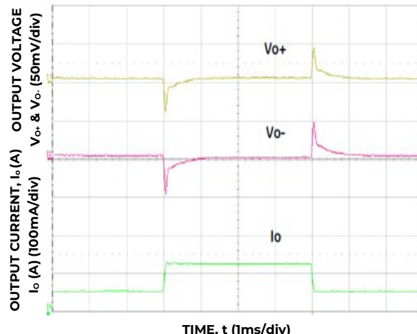
Figure 4. Transient Response to 0.1A/ \mu s Dynamic Load Change from 50% to 75% to 50% of full load, V_{in}=24V .
