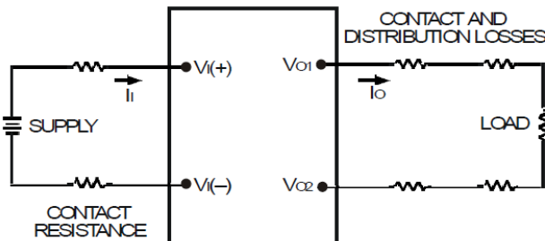
Figure 12. Output Ripple and Noise Test Setup.
