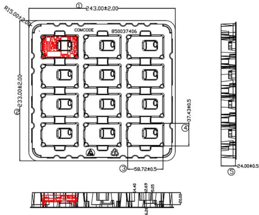
Base Plate Module Tray
