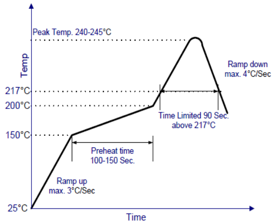
Figure 22. Recommended linear reflow profile using Sn/Ag/Cu solder
