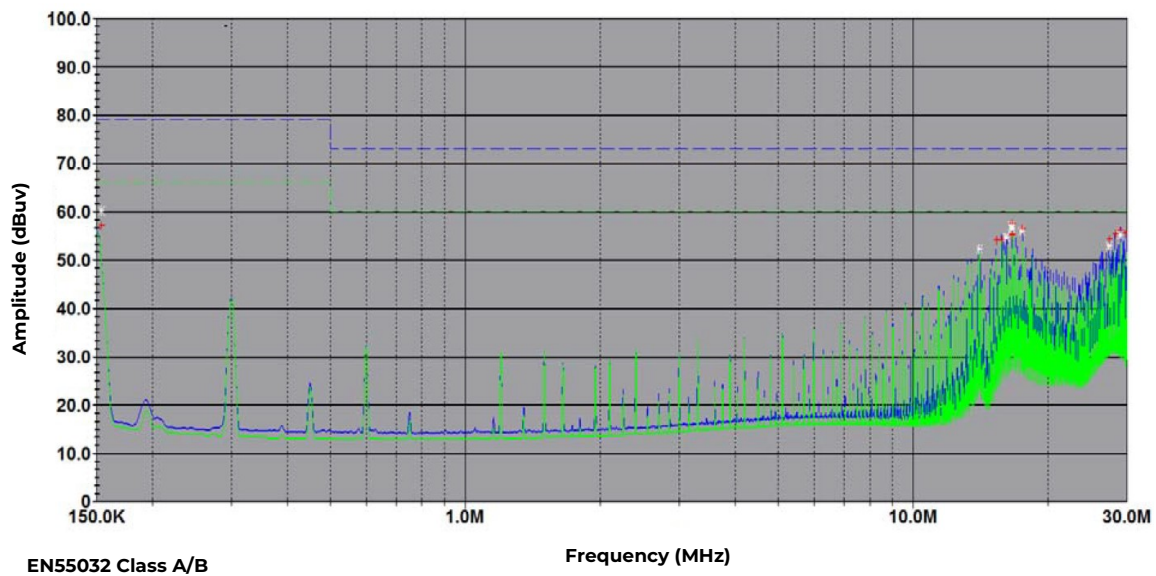
Figure 23. EMC Consideration
