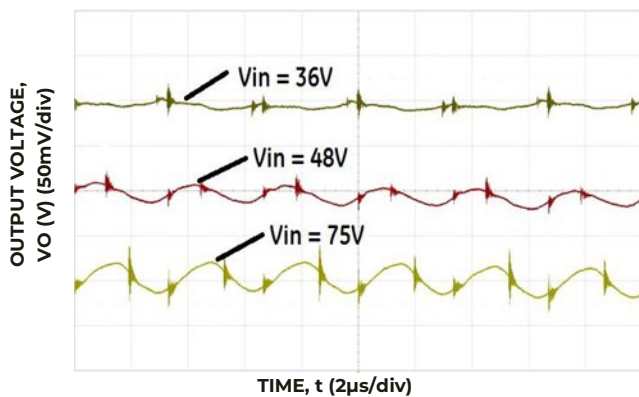
Figure 3. Typical Output Ripple and Noise, I_o = I_{o,max} , C_o = C_{o,min}
