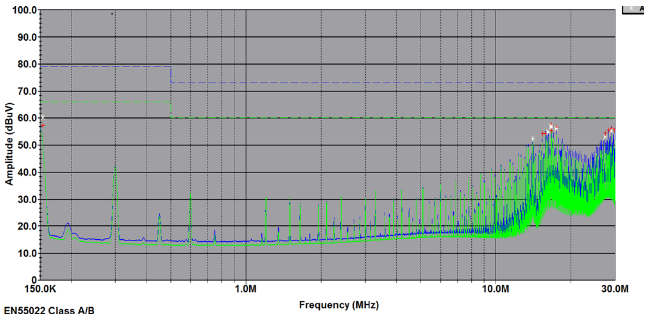
Figure 24. EMC Consideration
