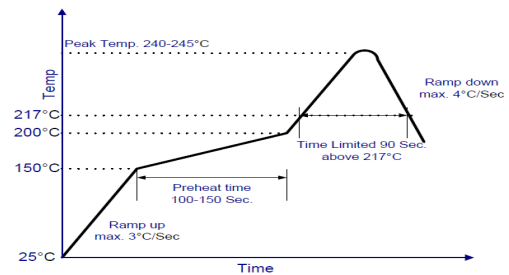
Figure 22. Recommended linear reflow profile using Sn/Ag/Cu solder.
