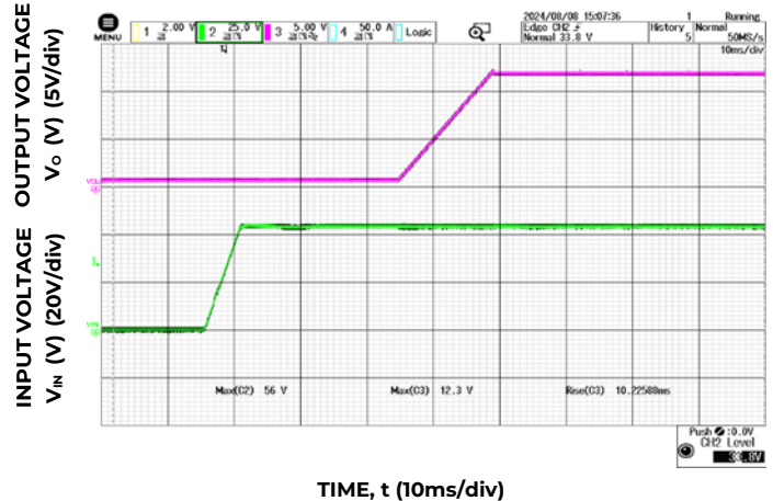
Figure 6. Typical Start-up Using Input Voltage ( V_{IN} = 54\text{V} , I_o = I_{o,max} )
