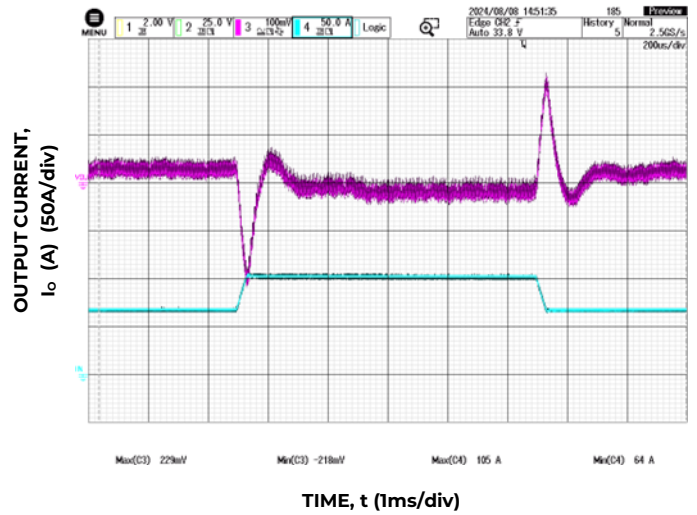
Figure 4. Dynamic Load Response, di_o/dt=1\text{A}/\mu\text{s} ; V_{IN}=V_{IN,nom} ; T_A=25^\circ\text{C} ; Load Change from I_o = 50\% to 75\% of I_{o,max} ; C_o = 250\mu\text{F} Ceramic + 3900\mu\text{F} PosCap Oscon
