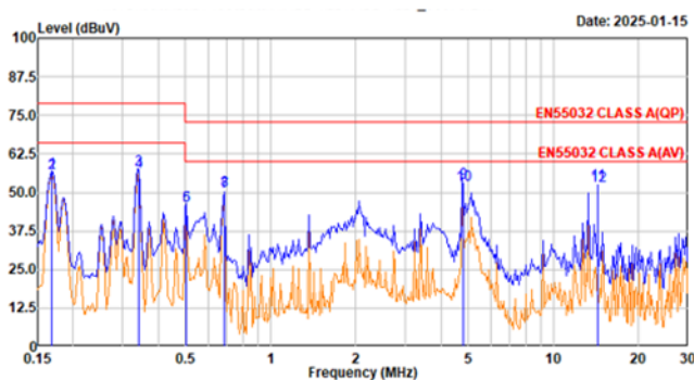
Figure 10. EMI with filter
