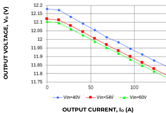
Figure 9. Typical Output Voltage Regulation vs Output Current with droop
