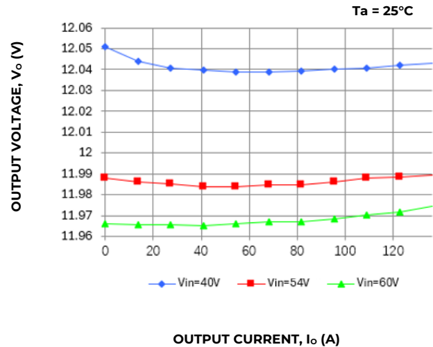
Figure 8. Typical Output Voltage Regulation vs Output Current
