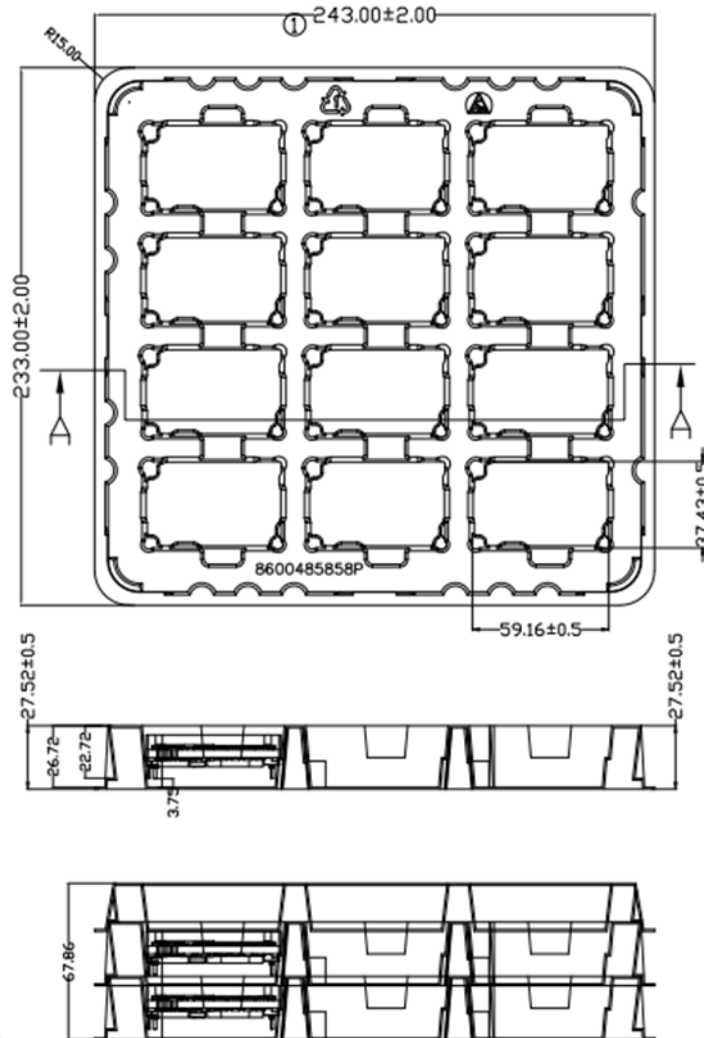
Figure 22. QODE136A0B Packaging Tray
