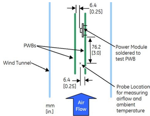
Figure 18. Thermal Test Setup
