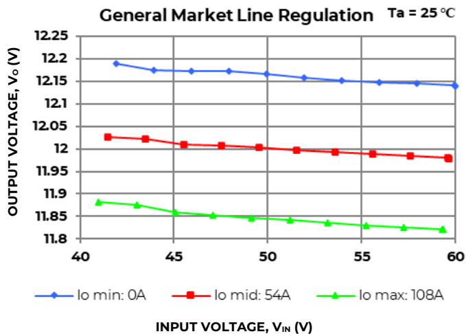
Figure 7. Typical Output Voltage Regulation vs Input Voltage, with droop
