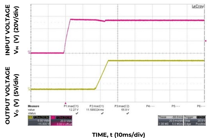
Figure 6. Typical Start-up Using Input Voltage ( V_{in} = 54\text{V} , I_o = 108\text{A} )
