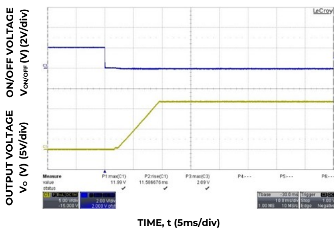
Figure 5. Typical Start-up Using On/Off Voltage ( I_o = 108\text{A} )
