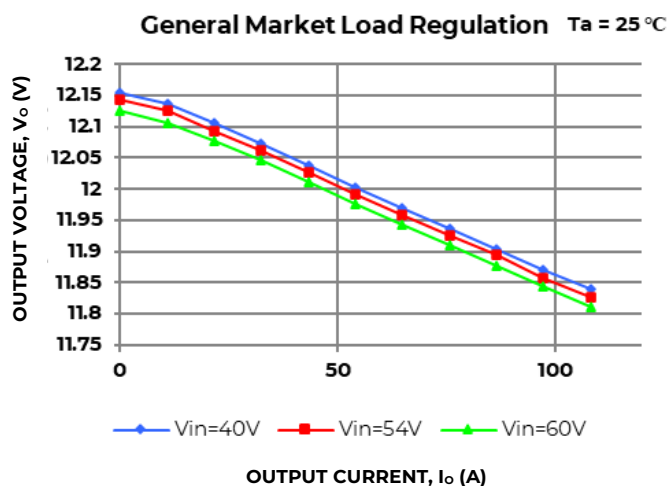
Figure 8. Typical Output Voltage Regulation vs Output Current, with droop
