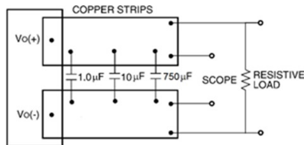
Figure 12. Output Ripple and Noise Test Setup.
