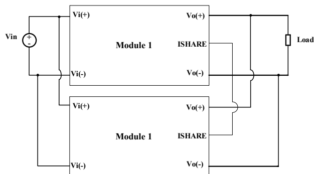
Figure 17. Parallel and active current sharing configuration.
