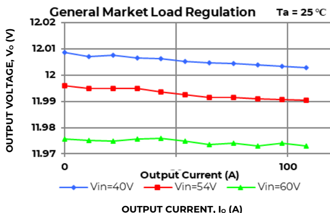
Figure 10. Typical Output Voltage Regulation vs Output Current, without droop
