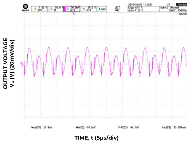
Figure 3. Typical output ripple and noise ( C_o = 650\mu\text{F} Ceramic + 470\mu\text{F} \times 2 PosCap Oscon, V_{in} = 54\text{V} , I_o = 108\text{A} )
