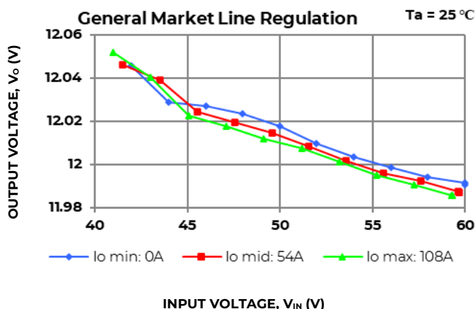
Figure 9. Typical Output Voltage Regulation vs Input Voltage, without droop
