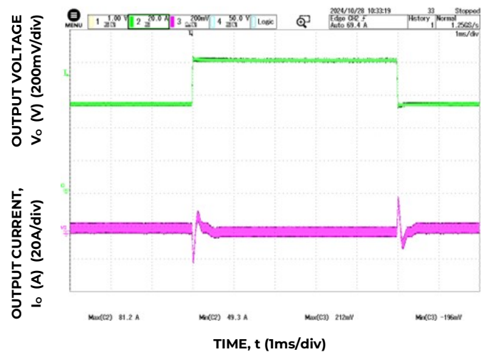
Figure 4. Dynamic Load Response, di_o/dt=1\text{A}/\mu\text{s} ; V_{in}=54\text{V} ; T_a=25^\circ\text{C} ; I_o = 50\% to 75\% of I_{o,max} ; C_o = 520\mu\text{F} Ceramic + 4680\mu\text{F} Ploy CAP
