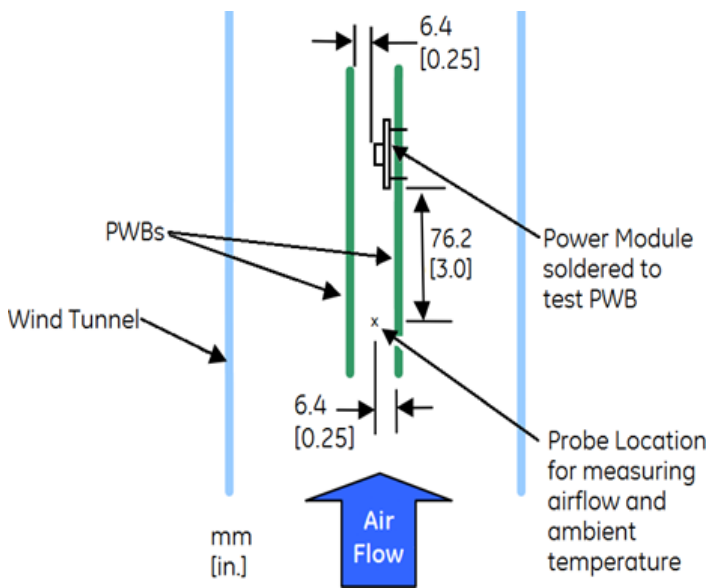
Figure 14. Thermal Test Setup
