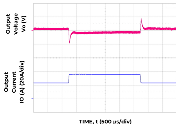
Figure 4. Typical Transient Response to 1A/ \mu s Step Change in Load from 50% to 75% to 50% of Full Load, C_O=1800\mu F and 50 Vdc Input
