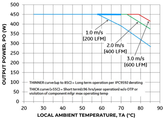
Figure 19. Output Power Derating for the QBVS046A9 S9R6-H Base Plate Option in the Longitudinal Orientation; Airflow Direction from Vout to Vin; = 50V
