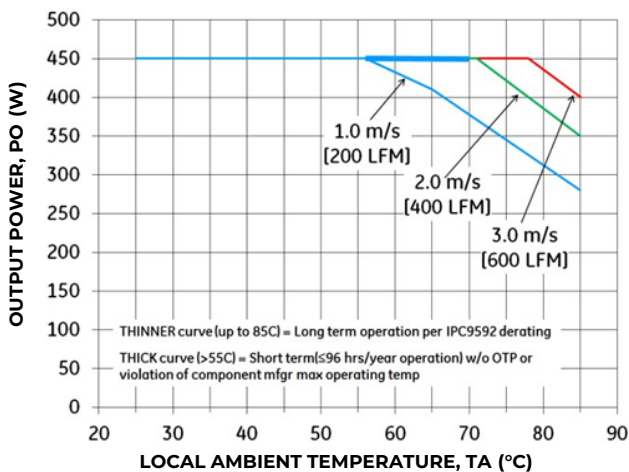
Figure 20. Output Power Derating for the QBVS046A9 S9R6-H Base Plate Option in the Longitudinal Orientation; Airflow Direction from Vout to Vin; = 55-55V
