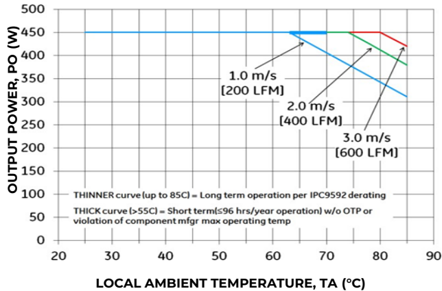
Figure 18. Output Power Derating for the QBVS046A9 S9R6-H Base Plate Option in the Longitudinal Orientation; Airflow Direction from Vout to Vin; = 45V
