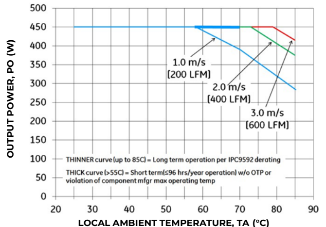
Figure 17. Output Power Derating for the QBVS046A9 S9R6-H Base Plate Option in the Transverse Orientation; Airflow Direction from Vin(-) to Vin(+); Vin = 54-55V
