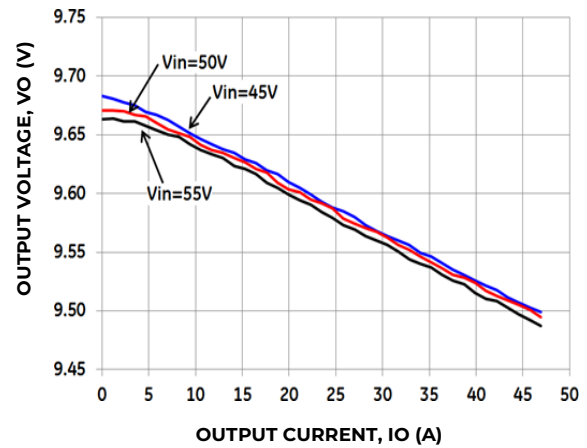
Figure 8. Typical Output Voltage Regulation vs. Output Current for the -P Version
