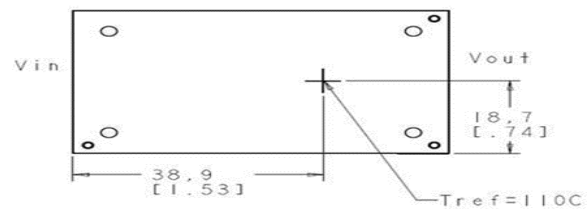
Figure 13. Location of the thermal reference temperature Tref
