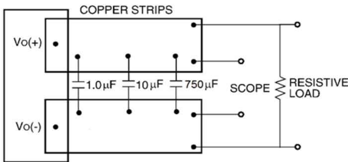
Figure 10. Output Ripple and Noise Test Setup
