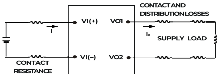
Figure 11. Output Voltage and Efficiency Test Setup
