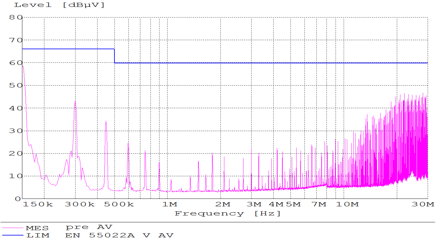
Figure 22. EMC Consideration
