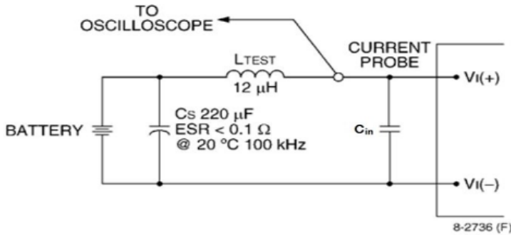
Figure 9. Input Reflected Ripple Current Test Setup
