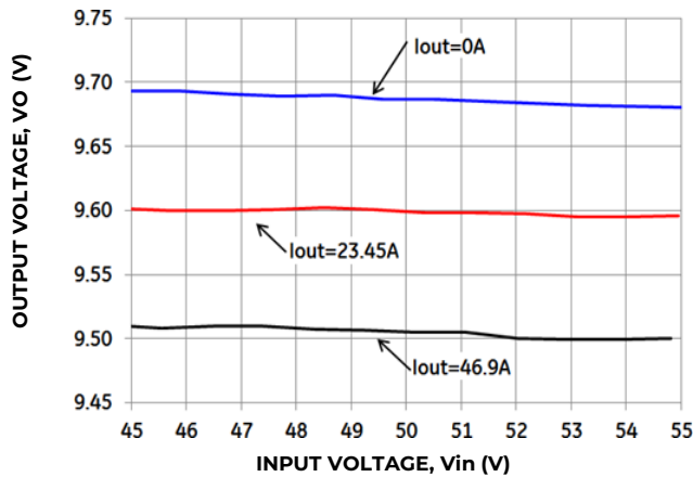
Figure 7. Typical Output Voltage Regulation vs. Input Voltage the -P Version
