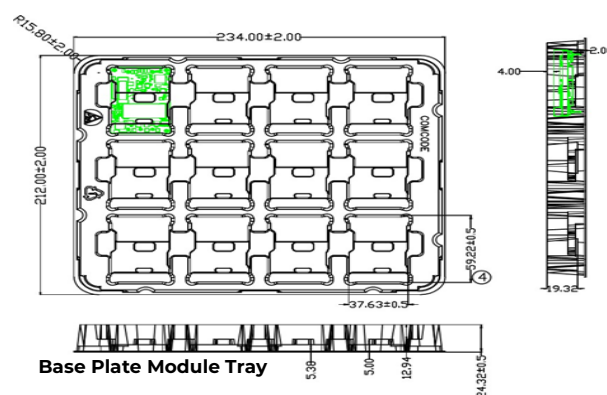
Figure 23. QBVS046A9S9R6 Packaging Tray
