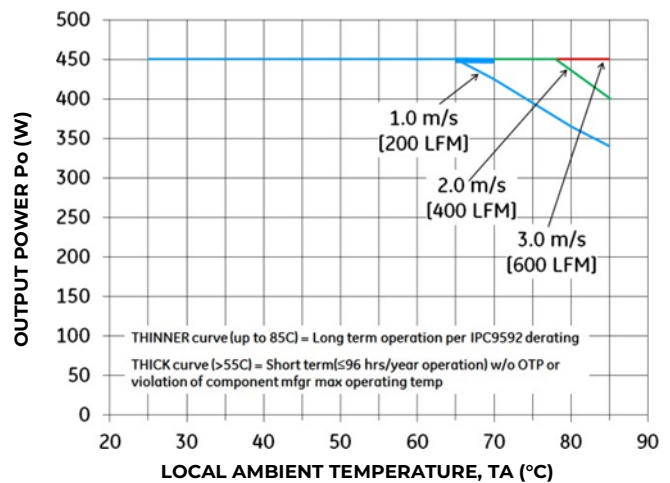
Figure 16. Output Power Derating for the QBVS046A9 S9R6-H Base Plate Option in the Transverse Orientation; Airflow Direction from Vin(-) to Vin(+); Vin = 50V
