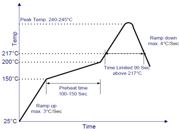
Figure 21. Recommended linear reflow profile using Sn/Ag/Cu solder
