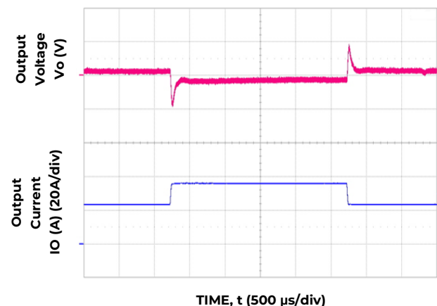
Figure 4. Typical Transient Response to 1A/μs Step Change in Load from 50% to 75% to 50% of Full Load, CO=1800\mu F and 50 Vdc Input
