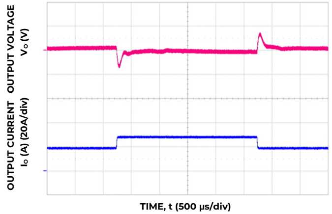
Figure 4. Typical Transient Response to 1A/μs StepChange in Load from 50% to 75% to 50% of Full Load, C_o=1200\mu\text{F} and 50 V dc Input
