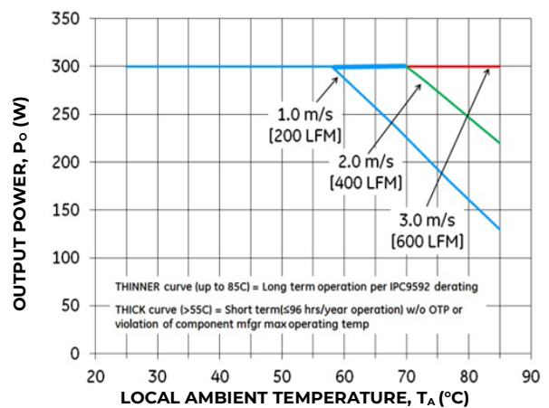
Figure 20. Output Power Derating for the Open Frame QBVK031A3S9R6 in the Longitudinal Orientation; Airflow Direction from V_{out} to V_{in} ; V_{in} = 55V .
