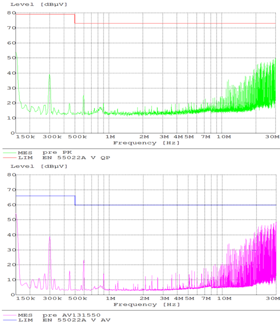
Figure 22. EMC Considerations
