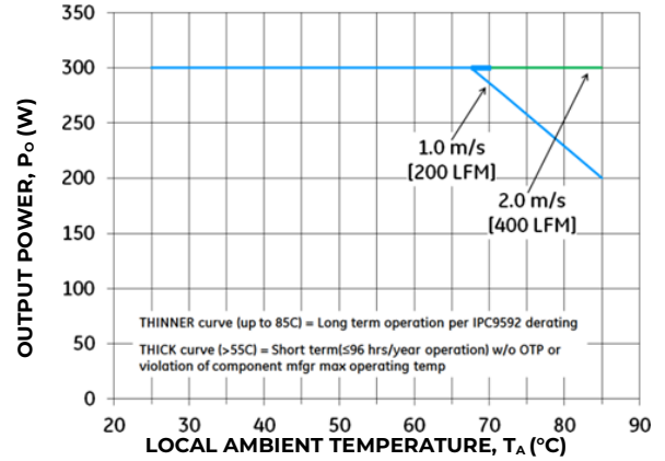
Figure 18. Output Power Derating for the Open Frame QBVK031A3S9R6 in the Longitudinal Orientation; Airflow Direction from V_{out} to V_{in} ; V_{in} = 38 to 42V .
