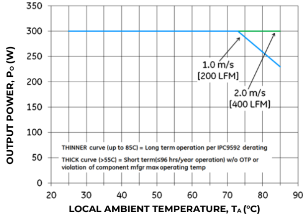
Figure 15. Output Power Derating for the Open Frame QBVK031A3S9R6 in the Transverse Orientation; Airflow Direction from V_{in}(-) to V_{in}(+) ; V_{in} = 38 to 42V .
