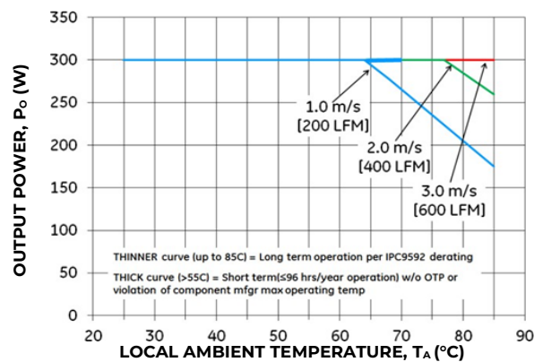
Figure 19. Output Power Derating for the Open Frame QBVK031A3S9R6 in the Longitudinal Orientation; Airflow Direction from V_{out} to V_{in} ; V_{in} = 50V .
