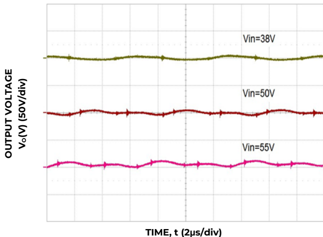
Figure 3. Typical Output Ripple and Noise, I_o = I_{o,max} C_o=750\mu\text{F} .
