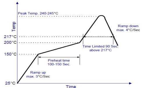
Figure 21. Recommended linear reflow profile using Sn/Ag/Cu solder.
