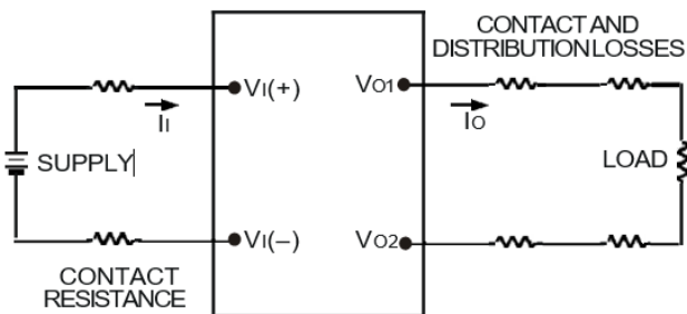
Figure 11. Output Voltage and Efficiency Test Setup.
