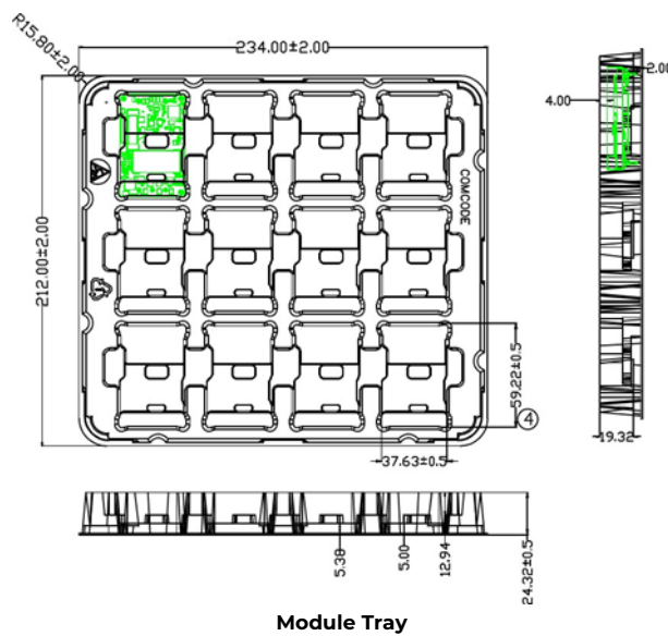
Figure 23. QBVK031A3S9R6 Packaging Tray
