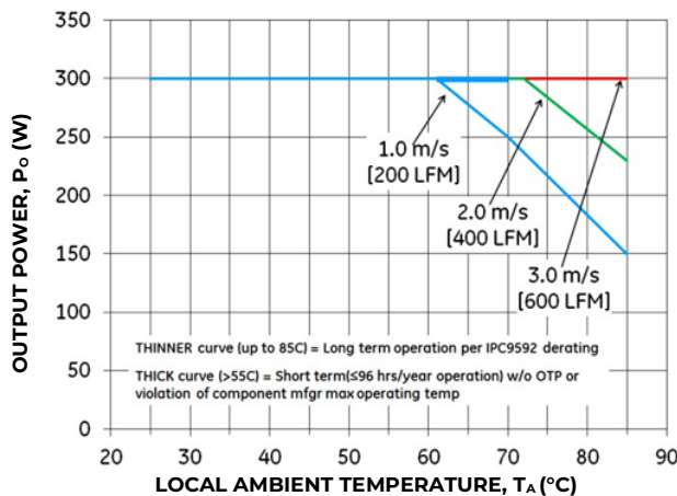
Figure 17. Output Power Derating for the Open Frame QBVK031A3S9R6 in the Transverse Orientation; Airflow Direction from V_{in}(-) to V_{in}(+) ; V_{in} = 55V .
