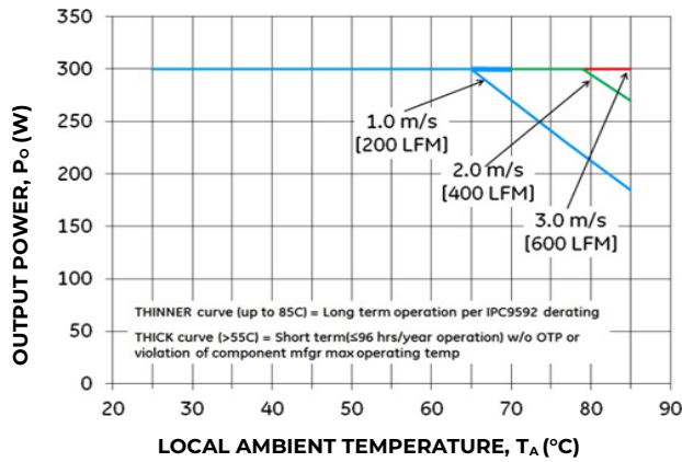
Figure 16. Output Power Derating for the Open Frame QBVK031A3S9R6 in the Transverse Orientation; Airflow Direction from V_{in}(-) to V_{in}(+) ; V_{in} = 50V .
