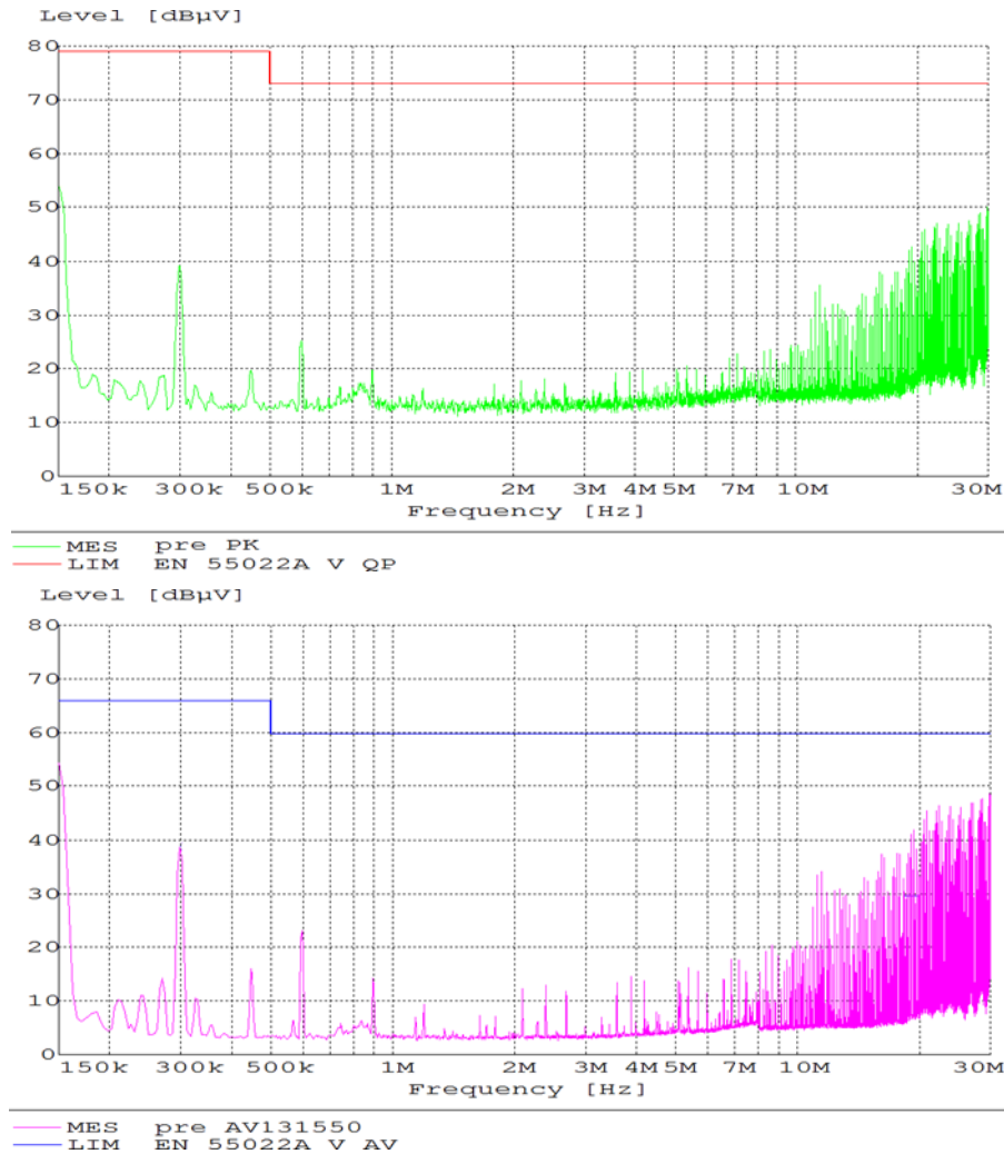
Figure 22. EMC Considerations
