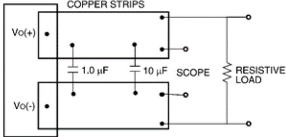
Figure 10. Output Ripple and Noise Test Setup 8-3299 (F)
