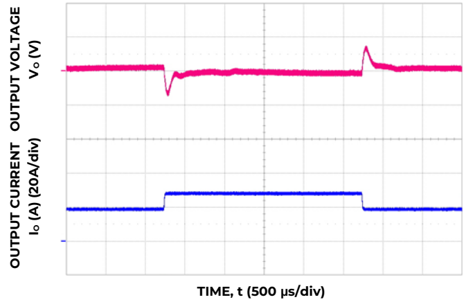
Figure 4. Typical Transient Response to 1A/μs StepChange in Load from 50% to 75% to 50% of Full Load, C_o = 1200\mu F and 50 V dc Input
