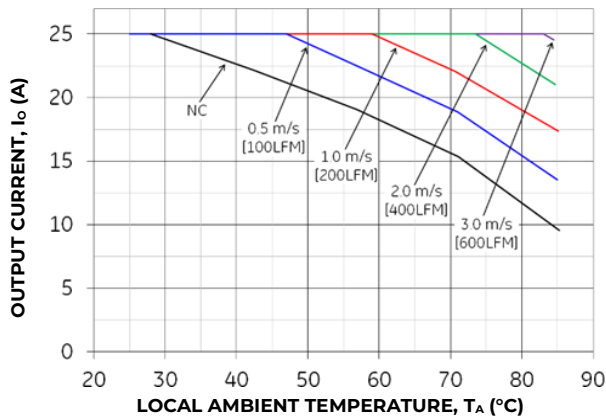
Figure 19. Output Current Derating for the Open Fram QBVW033A0B at 48V in with Transverse airflow from V_{in(-)} to V_{in(+)}
