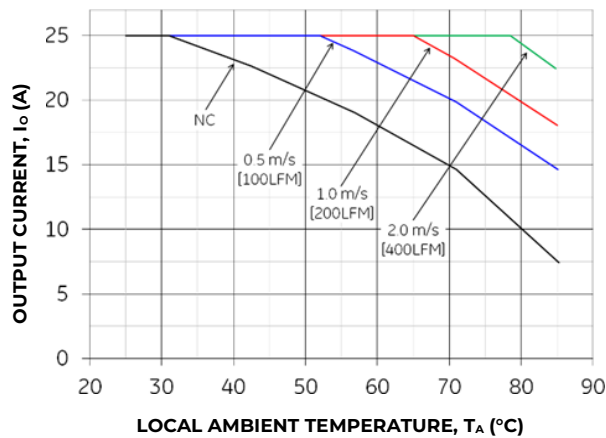
Figure 20. Output Current Derating for the Base plate QBVW033A0B-H at 48V in with Transverse airflow from V_{in(-)} to V_{in(+)}
