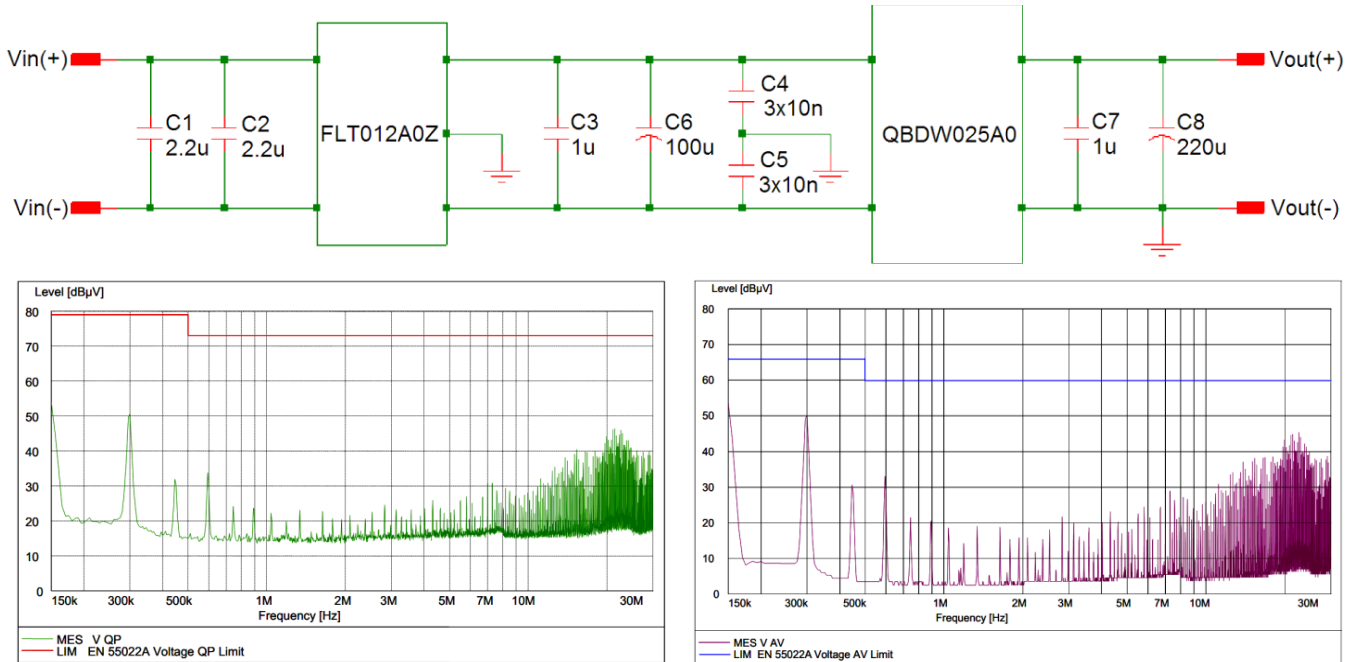
Figure 25. EMC Consideration
