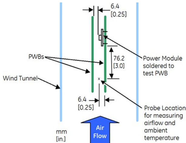
Figure 23. Thermal Test Setup
