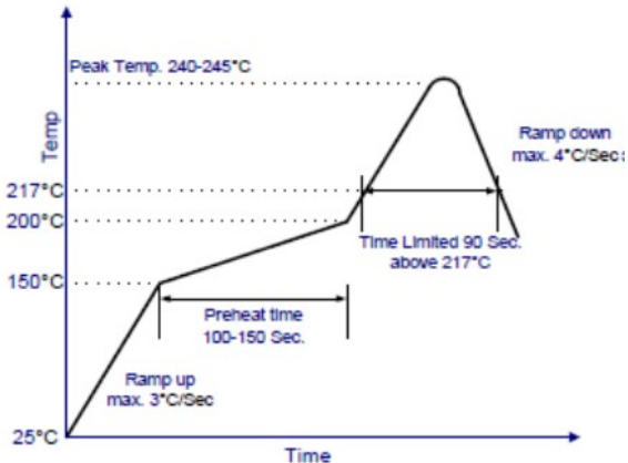
Figure 19. Recommended linear reflow profile using Sn/Ag/Cu solder.
