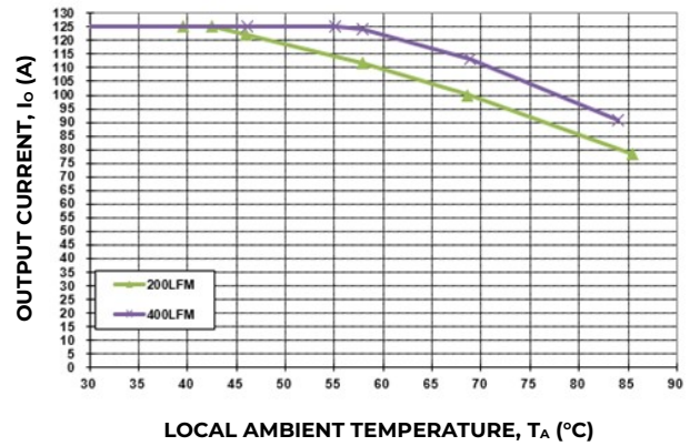
Figure 18. Output Current Derating for the Base plate QBDS125A10R4-H+0.6" Heat Sink; Airflow Direction for Vout to Vin (Worst) orientation; Vin = 54V.
