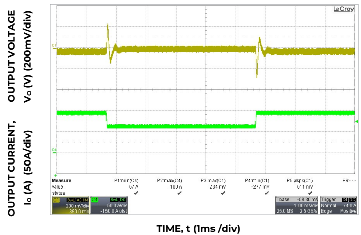
Figure 4. Dynamic Load Response, dI o /dt=1A/us; V in =V in,nom ; T A =25°C; Load Change from I o = 50% to 75% of I o,max ; C o =5200uF Ceramic;
