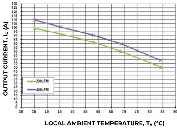
Figure 15. Output Current Derating for the Base Plate QBDS125A10R4-H; Airflow Direction for Vout to Vin(Worst) orientation; Vin = 50V.
