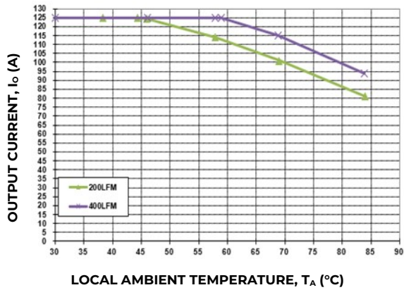
Figure 17. Output Current Derating for the Base plate QBDS125A10R4-H+0.6" Heat Sink; Airflow Direction for Vout to Vin (Worst) orientation; Vin = 50V.
