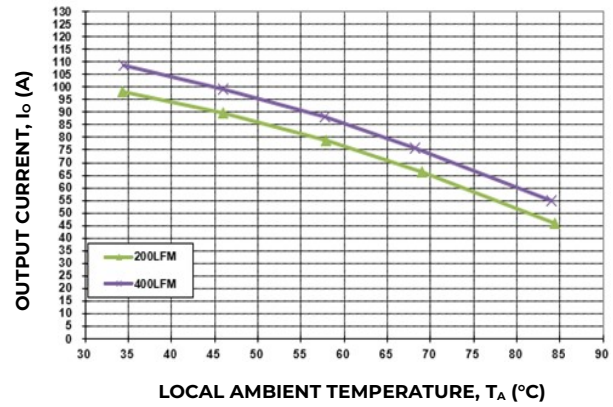
Figure 16. Output Current Derating for the Base Plate QBDS125A10R4-H; Airflow Direction for Vout to Vin(Worst) orientation; Vin = 54V.
