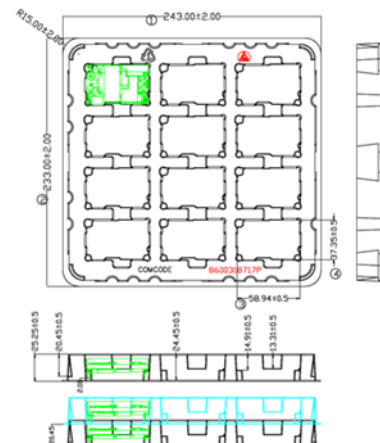
QBDS108A0B41 Packaging Tray
