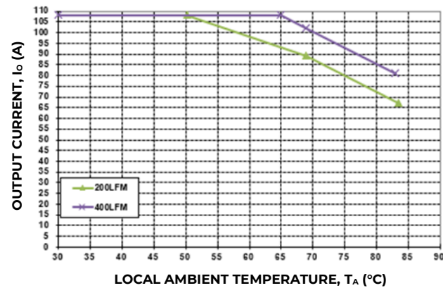
Figure 18. Output Current Derating for the Base plate QBDS108A0B-H+0.6" Heat Sink; Airflow Direction for Vout to Vin(Worst) orientation; Vin = 54V.
