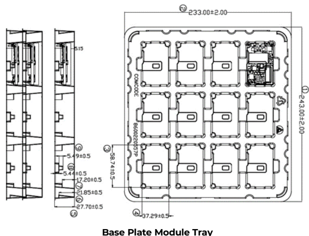
Figure 27. QBDE055A0B Packaging Tray
