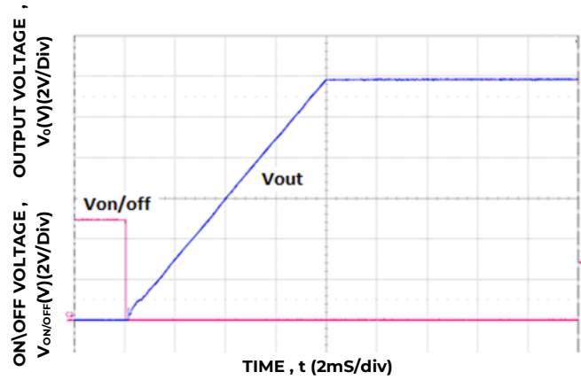
Figure 8. Typical Start-Up Using Remote On/Off with V_{in} applied, negative logic version, with the -P option shown, I_o = 33.5 I_{o,max} .
