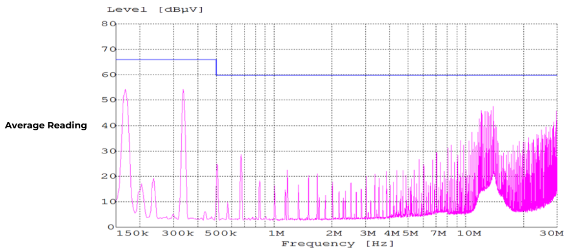
Figure 26 : EMC Consideration
