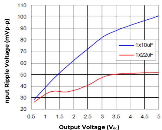
Figure 41. Input ripple voltage for various output voltages with 1 \times 10 \mu F or 1 \times 22 \mu F ceramic capacitors at the input (2A load). Input voltage is 12V. Scope BW: 20MHz
