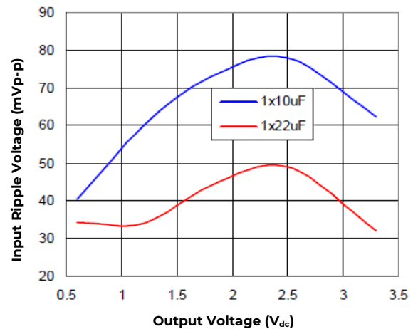
Figure 40. Input ripple voltage for various output voltages with 1 \times 10 \mu F or 1 \times 22 \mu F ceramic capacitors at the input (2A load). Input voltage is 5V. Scope BW: 20MHz.
