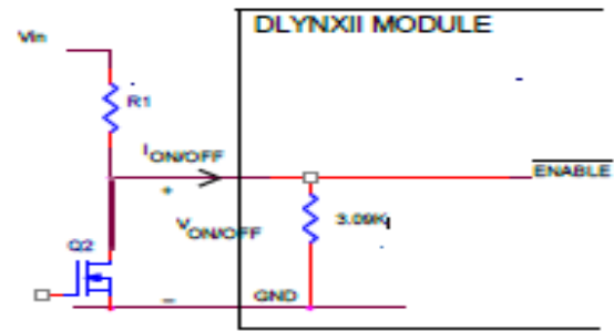
Figure 40. Circuit configuration for using negative On/Off logic.
