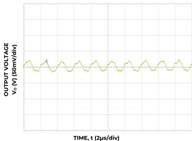
Figure 33. Typical output ripple and noise ( C_o=5 \times 22\mu\text{F} ceramic, V_{IN}=12\text{V} , I_o = I_{o,max} ).
