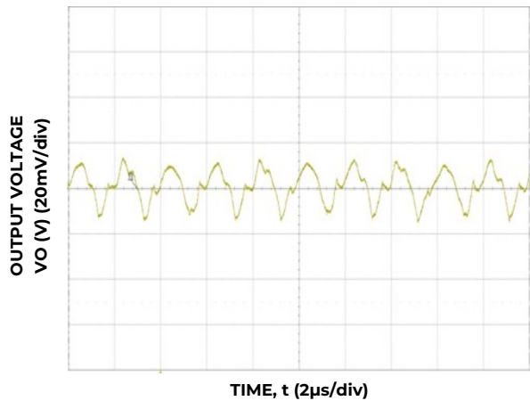
Figure 21. Typical output ripple and noise ( C_o=5 \times 22\mu\text{F} ceramic, V_{IN} = 12\text{V} , I_o = I_{o,max} ).
