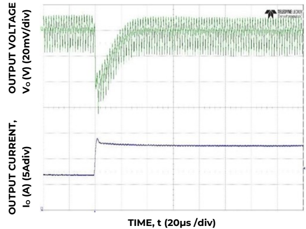
Figure 22. Transient Response to Dynamic Load Change from 50% to 100% at 12Vin, C_{out} = 4 \times 47\mu\text{F} + 1 \times 330\mu\text{F} CTune=1.2nF, RTune=300Ω
