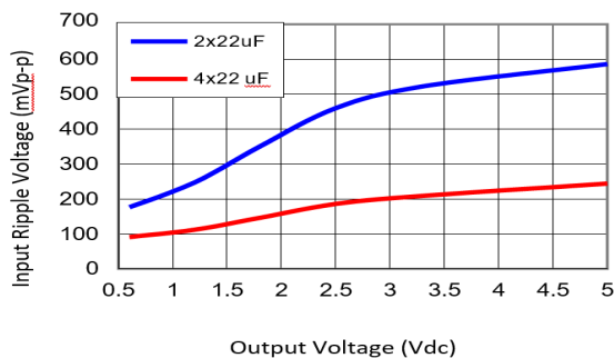
Figure 37. Input ripple voltage for various output voltages with 2x22 \mu F or 4x22 \mu F ceramic capacitors at the input (14A load). Input voltage is 12V.
