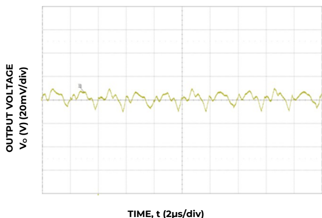
Figure 9. Typical output ripple ( C_o=5 \times 22\mu\text{F} ceramic, V_{IN} = 12\text{V} , I_o = I_{o,max} ).
