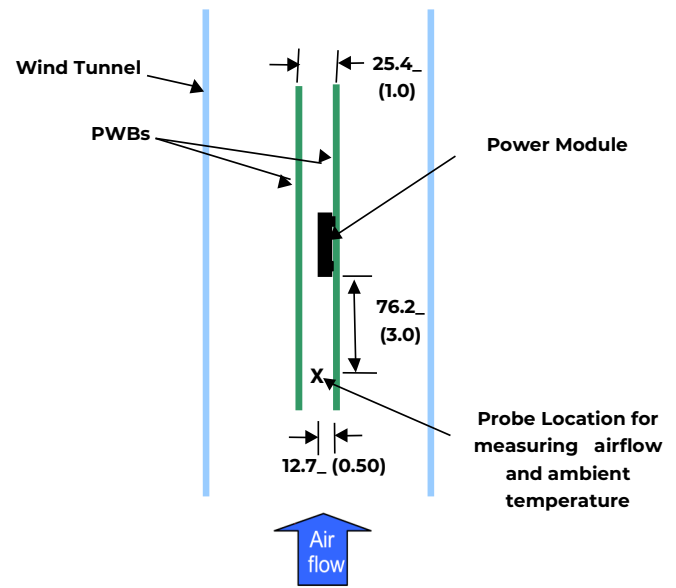
Figure 48. Thermal Test Setup.
