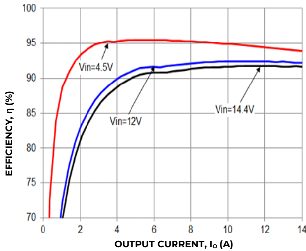
Figure 19. Converter Efficiency versus Output Current.
