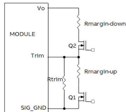
Figure 43. Circuit Configuration for margining Output voltage.
