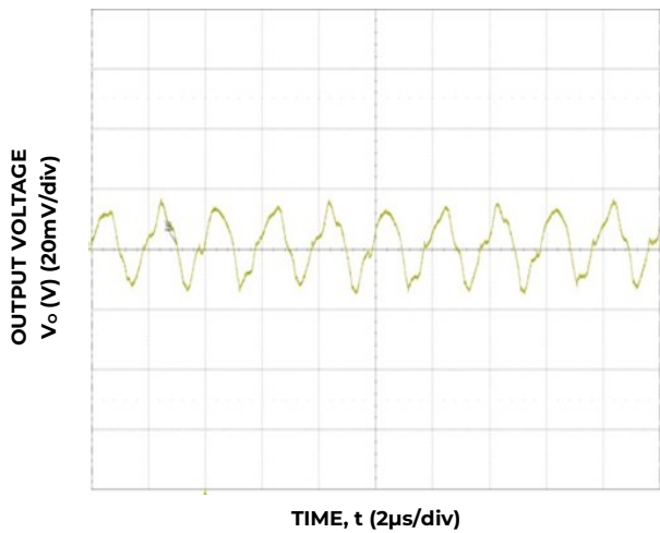
Figure 27. Typical output ripple and noise ( C_o=5 \times 22\mu\text{F} ceramic, V_{IN}=12\text{V} , I_o = I_{o,max} ).
