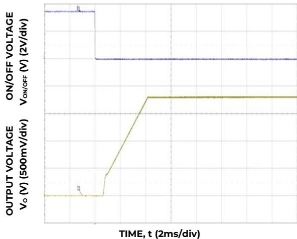
Figure 17. Typical Start-up Using On/Off Voltage ( I_o = I_{o,max} ).
