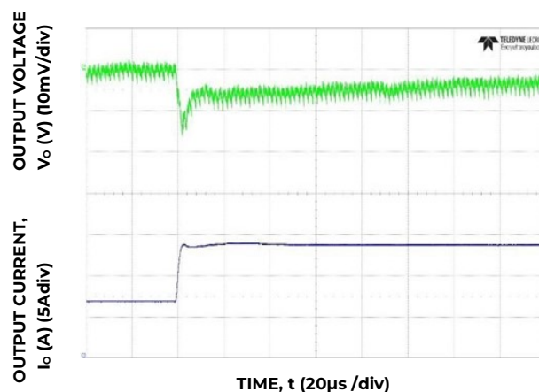
Figure 4. Transient Response to Dynamic Load Change from 50% to 100% at 12Vin, C_{out}=8 \times 47\mu\text{F}+8 \times 330\mu\text{F} C_{Tune}=27\text{nF} , R_{Tune}=300\Omega
