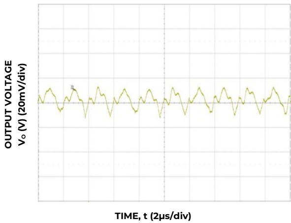
Figure 15. Typical output ripple and noise ( C_o=5X22\mu F ceramic, V_{IN}=12V , I_o = I_{o,max} ).
