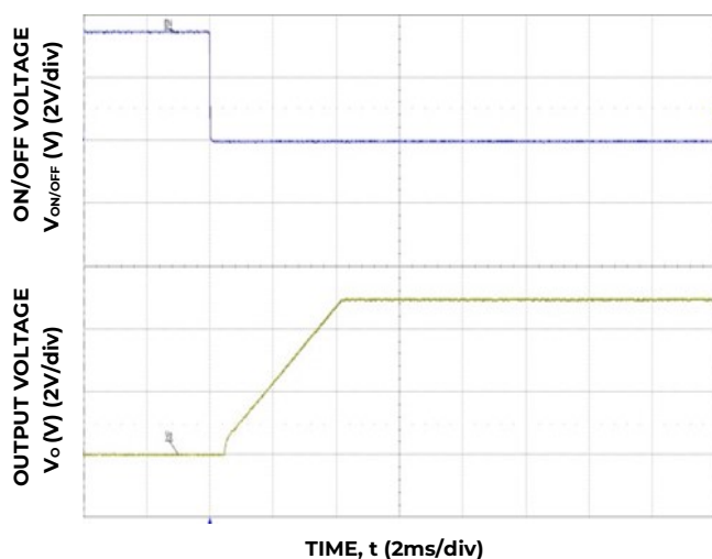
Figure 35. Typical Start-up Using On/Off Voltage ( I_o = I_{o,max} ).
