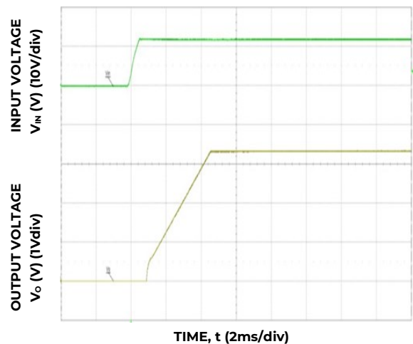
Figure 30. Typical Start-up Using Input Voltage ( V_{IN}=12\text{V} , I_o = I_{o,max} ).
