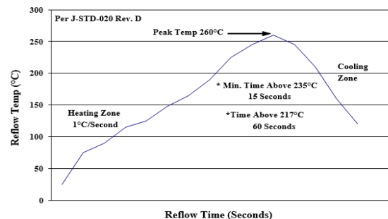
Figure 50. Recommended linear reflow profile using Sn/Ag/Cu solder.
