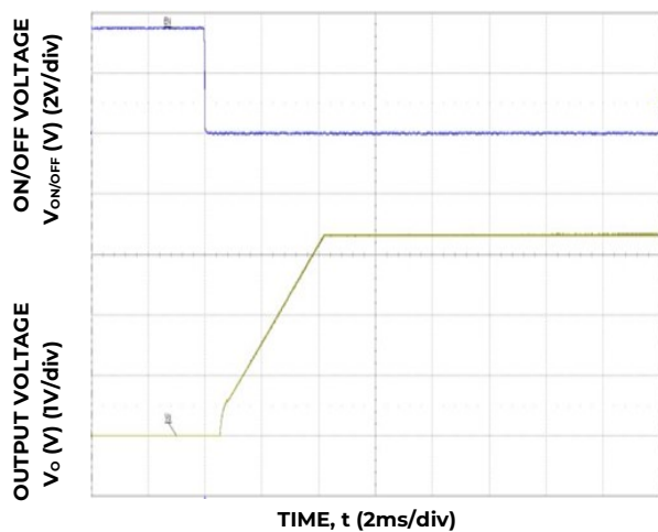
Figure 29. Typical Start-up Using On/Off Voltage ( I_o = I_{o,max} ).
