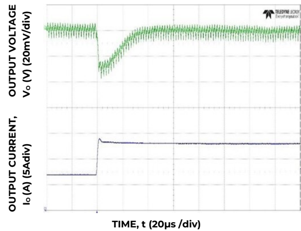
Figure 16. Transient Response to Dynamic Load Change from 50% to 100% at 12Vin, C_{out}=8x47\mu F+2x330\mu F CTune=1.8nF, RTune=300Ω
