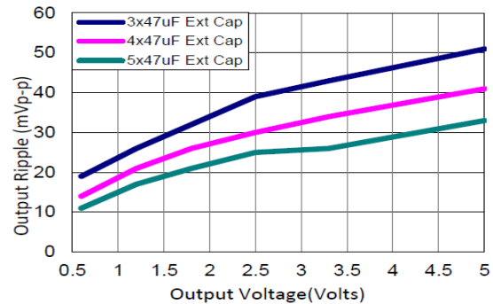
Figure 38. Output ripple voltage for various output voltages with external 3x47 \mu F, 4x47 \mu F or 5x47 \mu F ceramic capacitors at the output (14A load). Input voltage is 12V.
