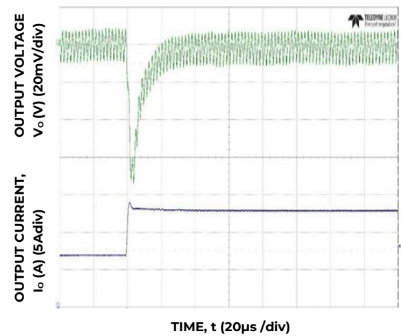
Figure 28 Transient Response to Dynamic Load Change from 50% to 100% at 12Vin, C_{out}=8 \times 47\mu\text{F} , C_{Tune}=1.2\text{nF} , R_{Tune}=300\Omega
