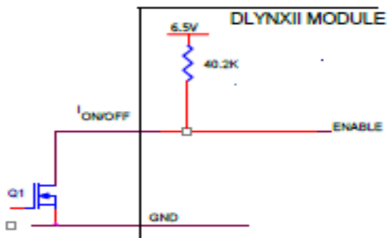
Figure 39. Circuit configuration for using positive On/Off logic.
