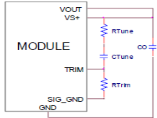
Figure 46. Circuit diagram showing connection of R_{TUNE} and C_{TUNE} to tune the control loop of the module.
