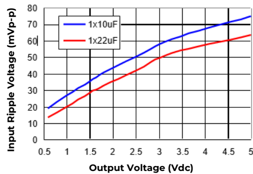
Figure 46. Input ripple voltage for various output voltages with 1 \times 10 \mu F or 1 \times 22 \mu F ceramic capacitors at the input (3A load). Input voltage is 12V
