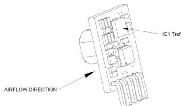
Figure 54. T_{ref} Temperature measurement location.
