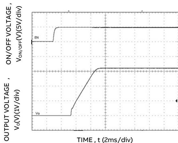
Figure 29. Typical Start-up Using On/Off Voltage ( I_o = I_{o,max} ).
