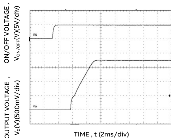
Figure 17. Typical Start-up Using On/Off Voltage (I o = I o,max ).
