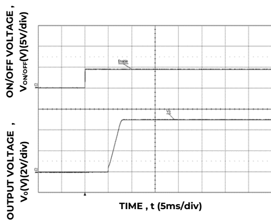
Figure 35. Typical Start-up Using On/Off Voltage ( I_o = I_{o,max}, V_{IN} = 12V, C_{ext} = 22\mu F ).
