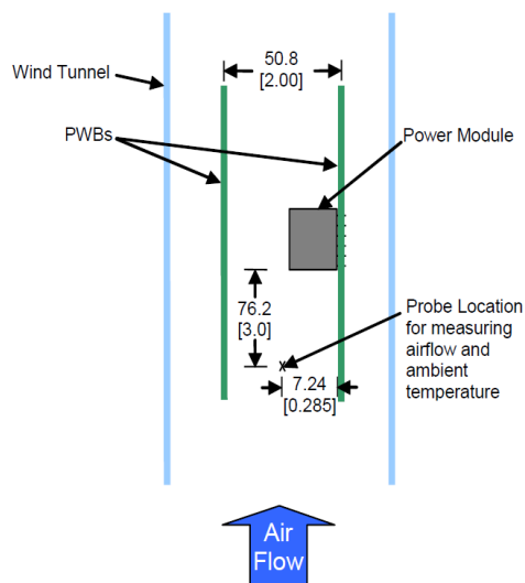
Figure 11 Thermal Test Set-up.
