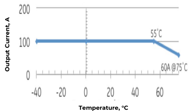
Rated Output Current (at V_{in} > 175V_{ac} )
