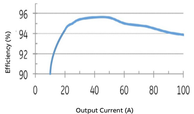
Efficiency % Typical at 240V ac
