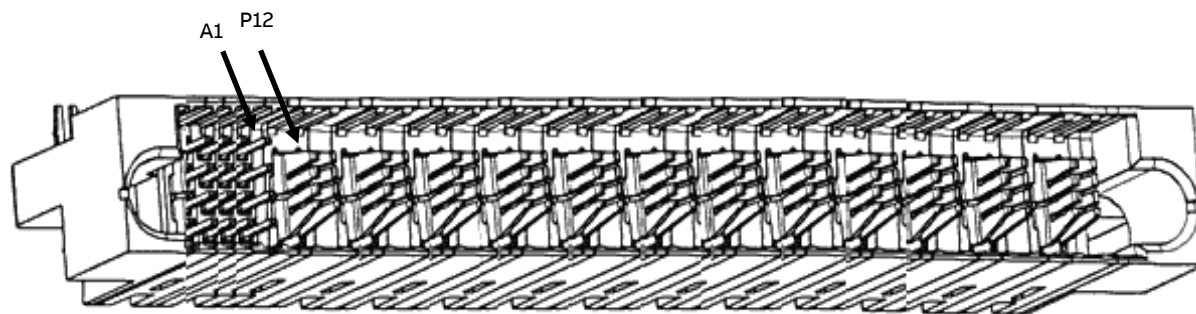
Power Unit Connector - AMP Multi-Beam XL (FCI # 51939-234LF or Tyco # 1900948-1)
