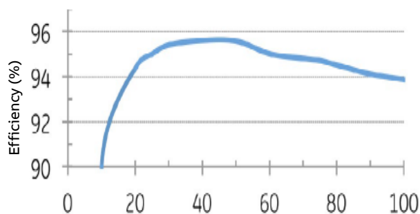
Efficiency % Typical at 240V ac
