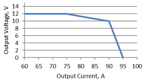
Current Limit Profile
