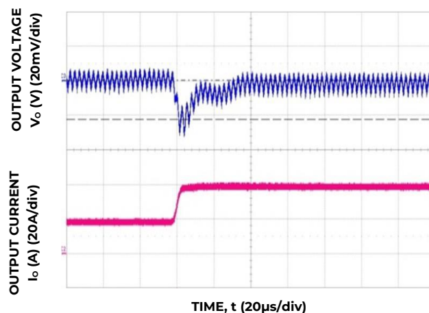
Figure 10. Transient Response to Dynamic Load Change from 50% to 100% at 12V in , C out = 6x330μF, C Tune =12nF, R Tune =200 ohms
