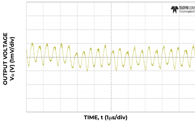
Figure 15. Typical output ripple ( C_o=4 \times 0.047 \mu\text{F} + 4 \times 0.1 \mu\text{F} + 15 \times 22 \mu\text{F} + 73 \times 47 \mu\text{F} + 6 \times 470 \mu\text{F} polymer, V_{IN} = 12\text{V} , I_o = I_{o,max} ).
