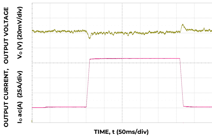
Figure 10. Trans. Resp. to 100A/μs Load Change from 25% to 75% at 12V IN , C_o=4 \times 0.047\mu\text{F} + 4 \times 0.1\mu\text{F} + 15 \times 22\mu\text{F} + 73 \times 47\mu\text{F} + 6 \times 470\mu\text{F} polymer.
