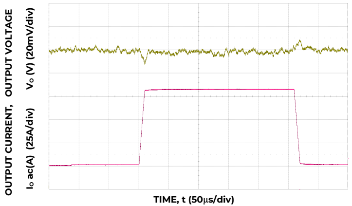
Figure 22. Trans. Resp. to 100A/µs Load Change from 25% to 75% at 12\text{V}_{IN} , C_o=4 \times 0.047\mu\text{F} + 4 \times 0.1\mu\text{F} + 15 \times 22\mu\text{F} + 73 \times 47\mu\text{F} + 6 \times 470\mu\text{F} polymer.
