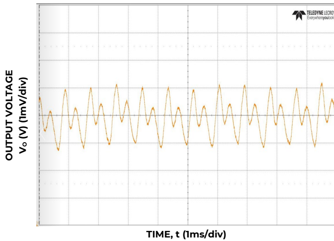
Figure 15. Typical output ripple (C o =4x0.047μF + 4x0.1μF + 15x22μF + 73x47μF + 6x470μF polymer, V IN = 12V, I o = I o,max ).
