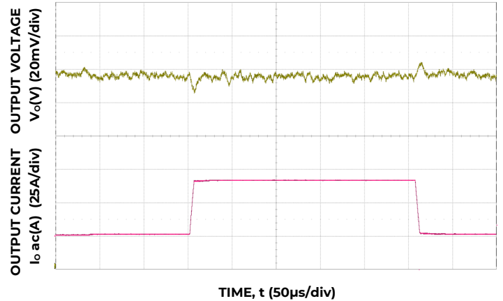
Figure 22. Trans. Resp. to 10A/ \mu\text{s} Load Change from 25% to 75% at 12VIN, C_o=4 \times 0.047\mu\text{F} + 4 \times 0.1\mu\text{F} + 15 \times 22\mu\text{F} + 73 \times 47\mu\text{F} + 6 \times 470\mu\text{F} polymer
