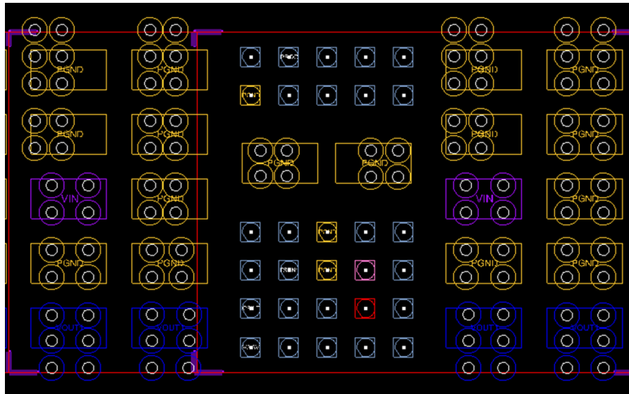
Figure 28. Example of Pad Layout with Vias
