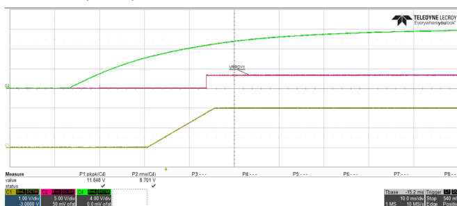
Figure 27. VIN, PGOOD1 and Vout1 waveform.
