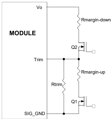
Figure 25. Circuit Configuration for margining Output voltage.
