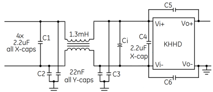
Figure 16. Suggested Configuration for EN55032 Class B.
