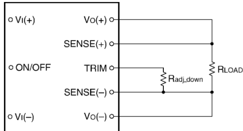
Figure 11. Circuit Configuration to Decrease Output Voltage.
