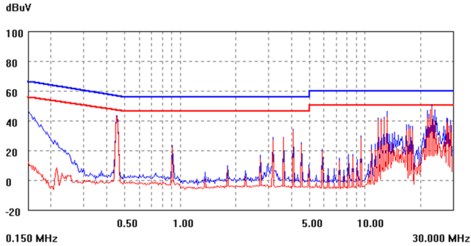
Figure 17. EMC signature using above filter, KSTW015A0F.
