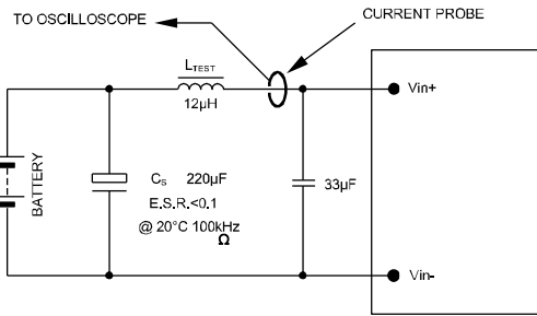
Figure 7. Input Reflected Ripple Current Test Setup.
