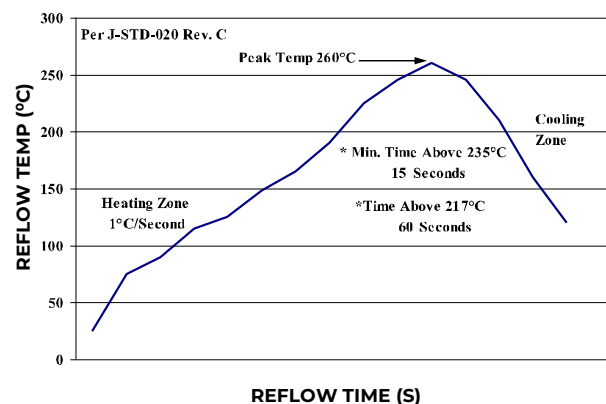
Figure 21. Recommended linear reflow profile using Sn/Ag/Cu solder.
