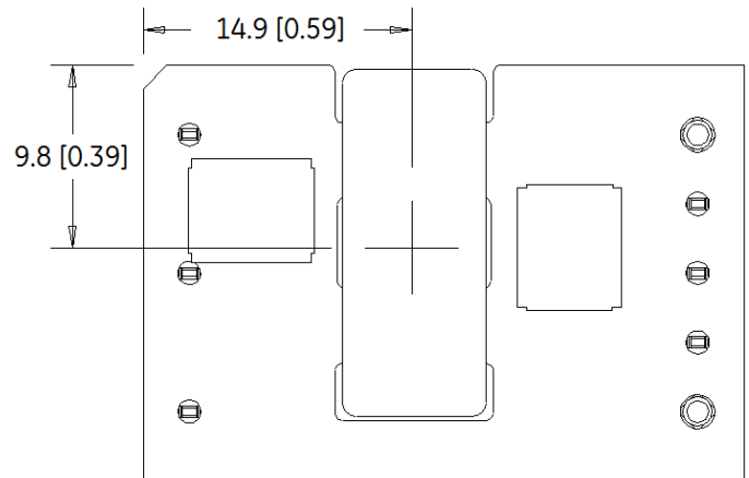
Figure 18. Pick and Place Location.
