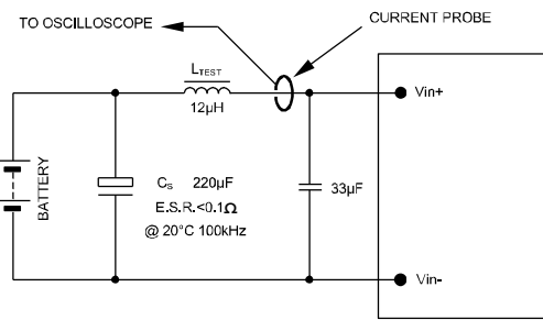
Figure 7. Input Reflected Ripple Current Test Setup.
