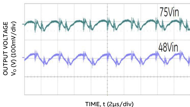
Figure 3. Typical output ripple and noise ( I_o = I_{o, max} ).
