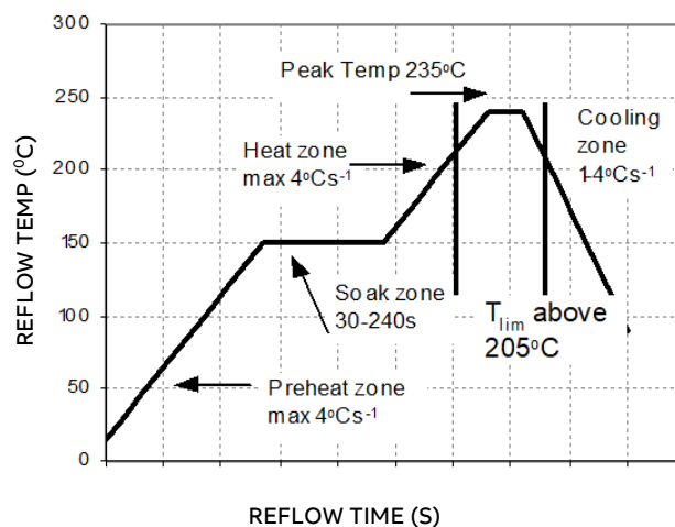
Figure 19. Recommended Reflow Profile for Sn/Pb solder.
