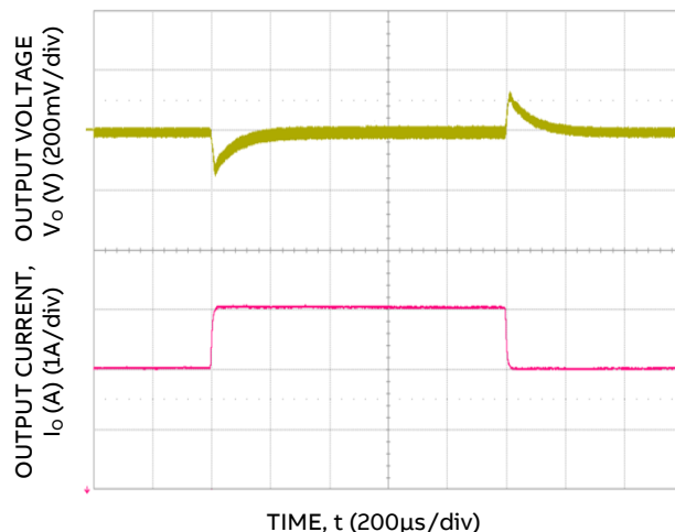
Figure 4. Transient Response to 0.1A/μS Dynamic load Change from 50% to 75% to 50% of full load, V_{in}=48V , C_o > 100μF
