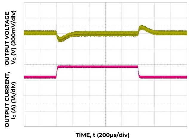
Figure 4. Transient Response to 0.1A/μS Dynamic Load Change from 50% to 75% to 50% of full load, V_{in}=48V , C_o > 100\mu F
