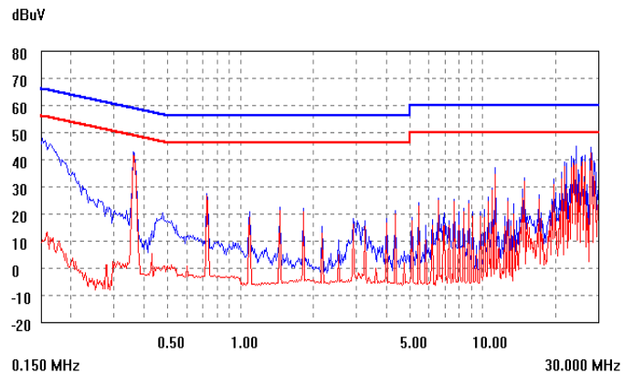
Figure 17. EMC signature using above filter, KSTW002A5B, V_{in}=48 V, Blue=PK, Red=Avg.
