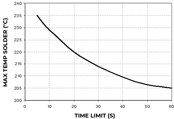
Figure 21. Time Limit, T_{lim} , Curve Above 205°C Reflow .
