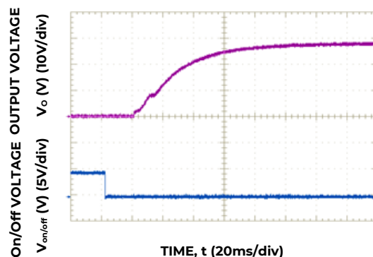
Figure 4. Typical Start-Up Using negative Remote On/Off; C_{o,ext} = 440\mu F .
