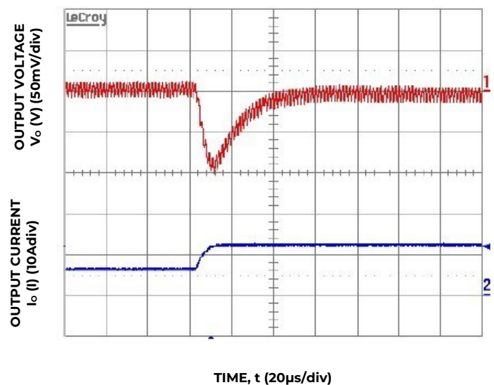
Figure 34. Transient Response to Dynamic Load Change from 50% to 100% at 12V IN , C out =5x47µF, C Tune =1500pF, R Tune =330ohms
