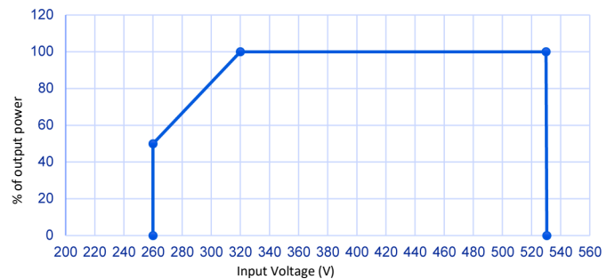
Fig.2 Input Limited Power Curve
