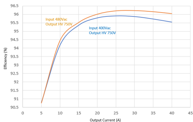
Fig.10 Rectifier Efficiency @ Output HV 750V
