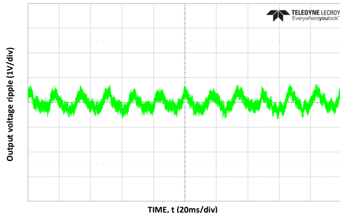
Fig.6 Output voltage ripple @Input 400Vac; Output HV 750V/Full load/ resistor load
