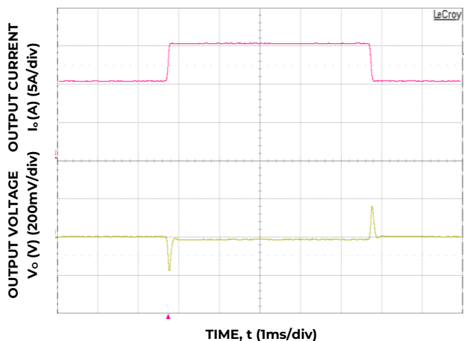
Figure 3. Transient Response to 0.1A/µs Dynamic Load Change from 50% to 75% to 50% of full load, V_{in}=48V
