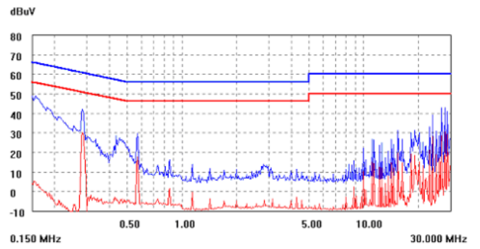
V_{IN} = 48V, I_o = I_{o,max}, N \text{ Line} Blue= Quasi-peak, Red = Avg
