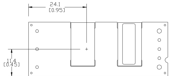
Figure 21. Pick and Place Location.
