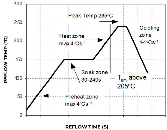
Figure 22. Reflow Profile for Tin/Lead (Sn/Pb) process.
