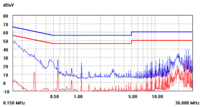
V_{IN} = 48V, I_o = I_{o,max}, L \text{ Line} Blue= Quasi-peak, Red = Avg
