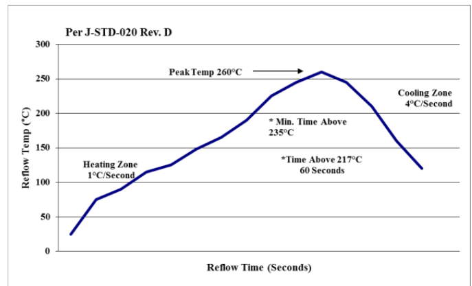
Figure 24. Recommended linear reflow profile using Sn/Ag/Cu solder.
