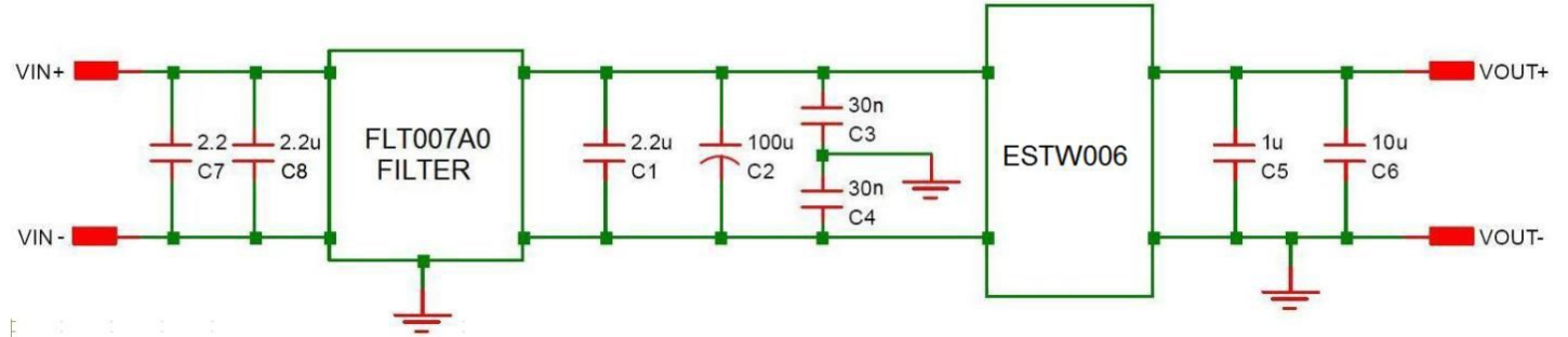
Figure 24. EMC Considerations
