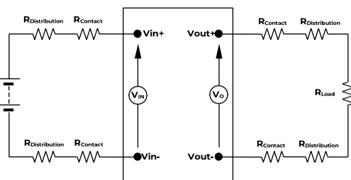
Figure 8. Output Voltage and Efficiency Test Setup
