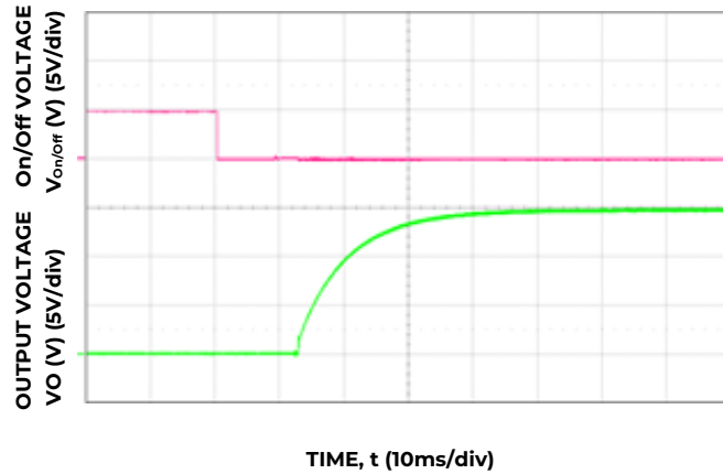
Figure 4. Typical Start-up Using Remote On/Off, negative logic version shown ( V_{IN} = 48V , I_o = I_{o,max} ).
