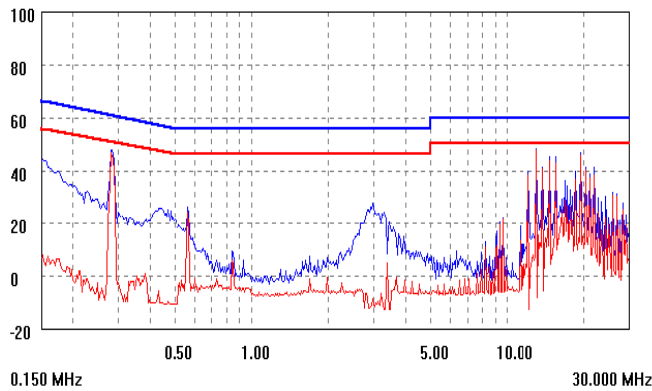
V IN = 48V, I o = I o,max , L Line
