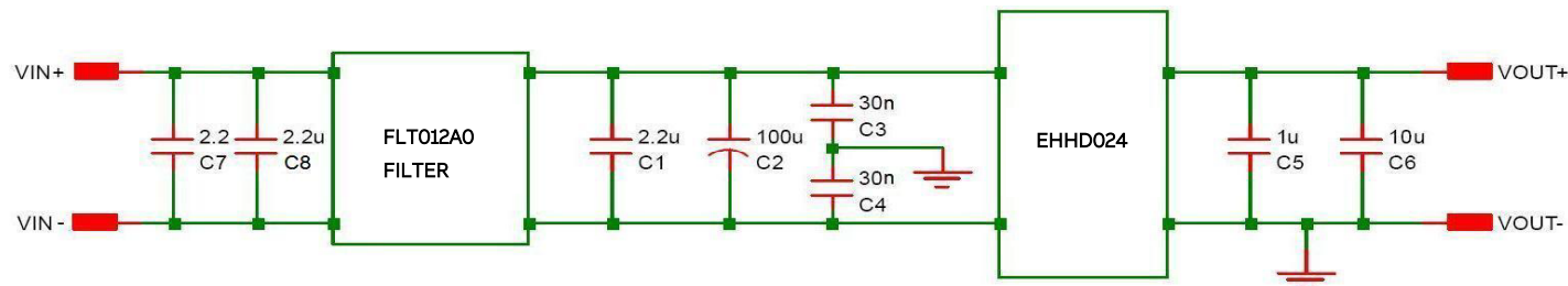
Figure 27. EMC Considerations
