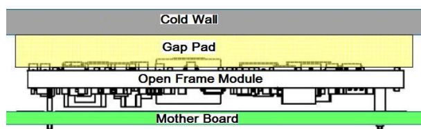
Figure 21. Cold Wall Mounting
