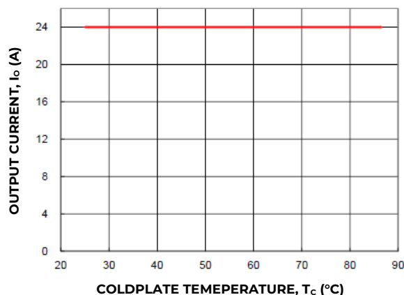
Figure 20. Derated Output Current versus Cold Wall Temperature with local ambient temperature around module at 85°C; V_{IN} = 24V or 48V.
