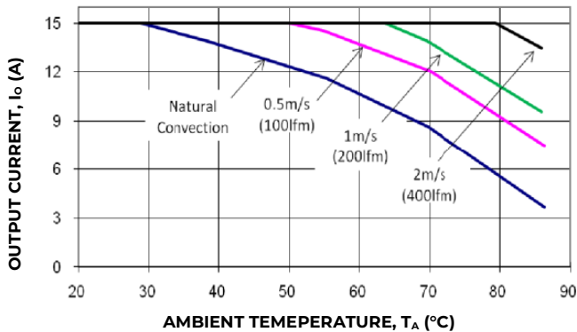
Figure 20. Output Current Derating for the Module with Heatplate; Airflow in the Transverse Direction for V_{out(-)} to V_{out(+)} ; V_{IN}=24V , V_O=5.0V .
