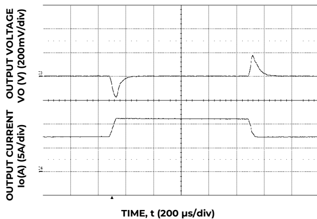
Figure 3. Transient Response to 0.1A/ \mu S Dynamic Load Change from 50% to 75% to 50% of full load, V_{in}=24V , C_o>100\mu F .
